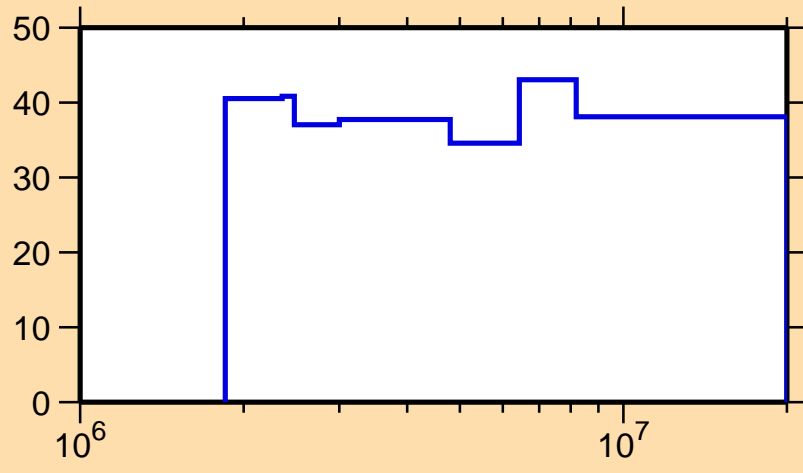
\Delta\sigma/\sigma vs. E for ^{203}\text{Au}(n, n_1)
