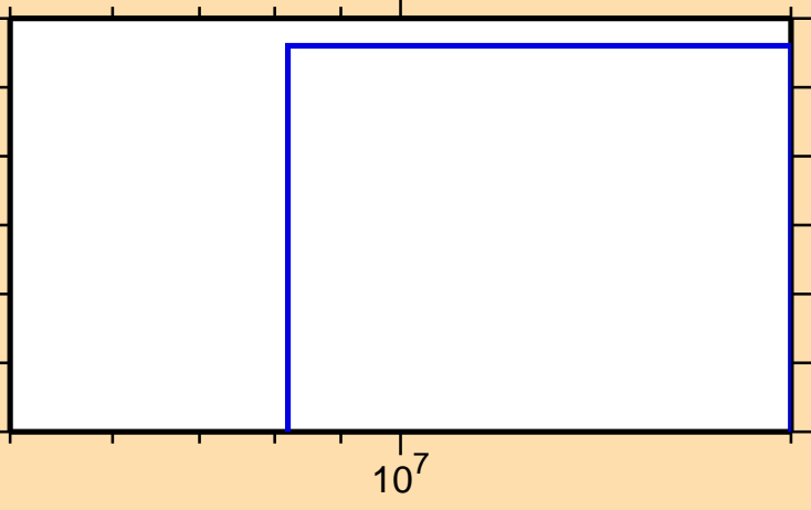
\sigma vs. E for ^{203}\text{Au}(n,d)
