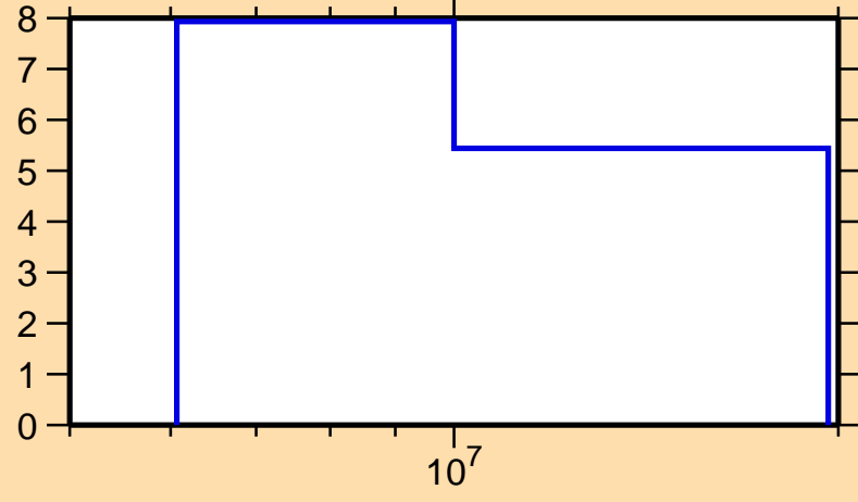
\Delta\sigma/\sigma vs. E for ^{205}\text{Au}(n,\text{tot.})
