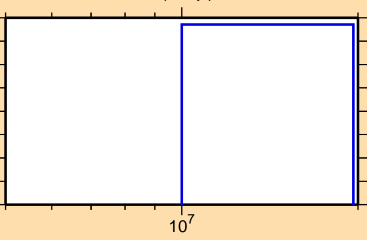
\sigma vs. E for ^{205}\text{Au}(n,np)
