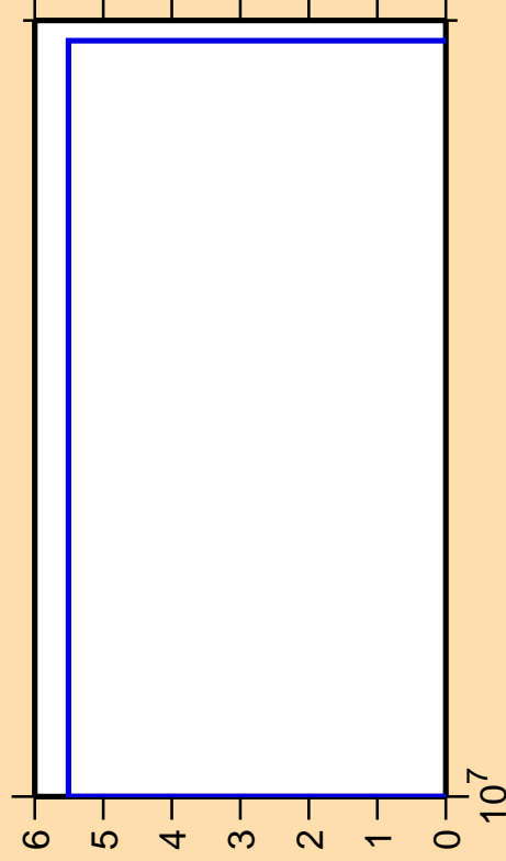
\Delta\sigma/\sigma vs. E for ^{205}\text{Au}(n,2np)
