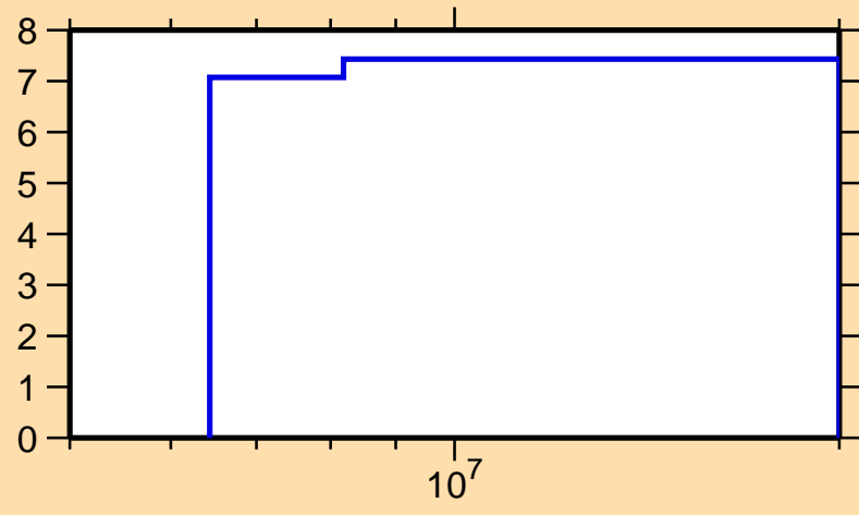
\Delta\sigma/\sigma vs. E for ^{205}\text{Au}(n,\text{el.})
