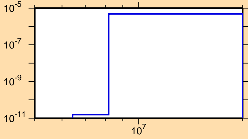
\sigma vs. E for ^{205}\text{Au}(n,\alpha)
