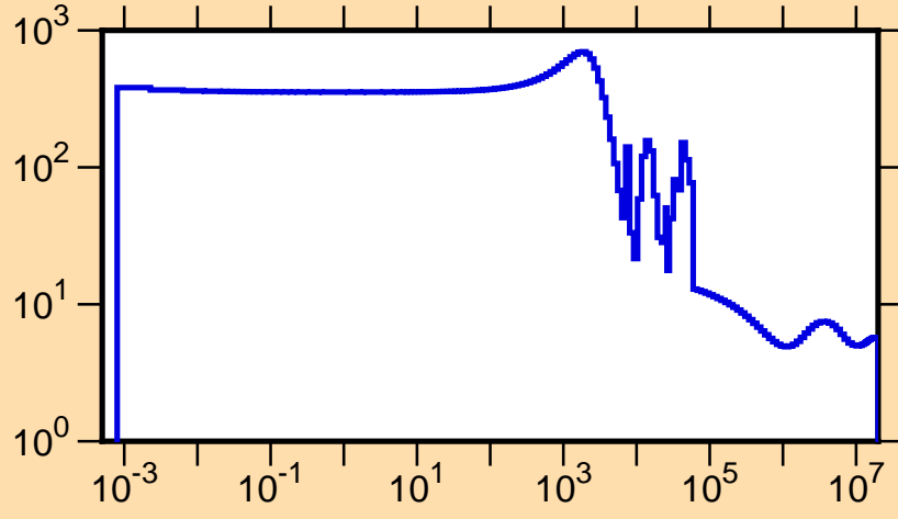
\sigma vs. E for ^{206}\text{Au}(n,\text{tot.})
