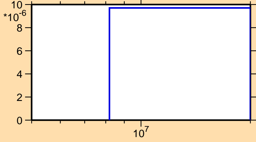
\sigma vs. E for ^{206}\text{Au}(n,d)
