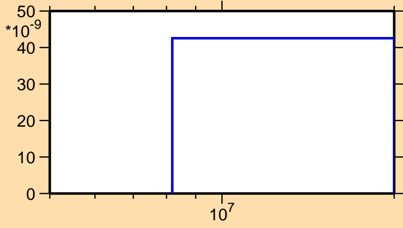
\sigma vs. E for ^{206}\text{Au}(n,nd)
