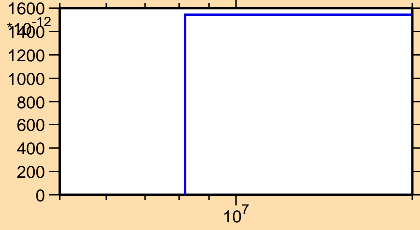
\sigma vs. E for ^{206}\text{Au}(n,2np)
