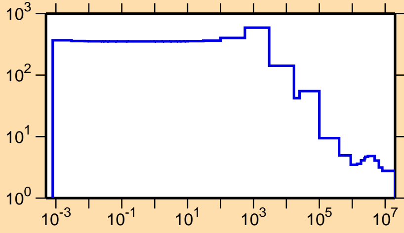
\sigma vs. E for ^{206}\text{Au}(n,\text{el.})
