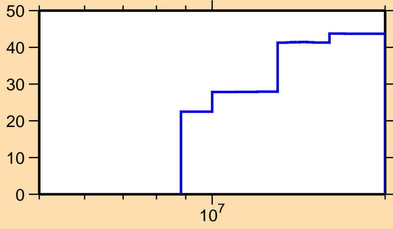
\Delta\sigma/\sigma vs. E for ^{207}\text{Au}(n,2n)
