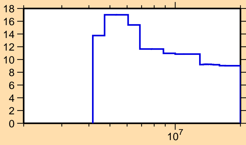
\Delta\sigma/\sigma vs. E for ^{207}\text{Au}(n,\text{nonel.})
