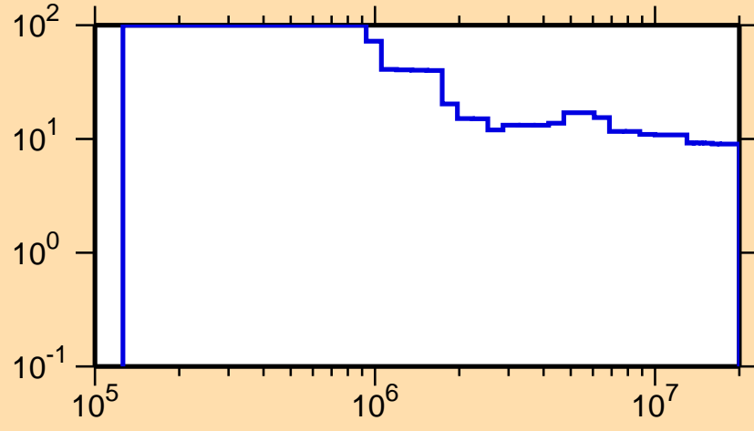
\Delta\sigma/\sigma vs. E for ^{207}\text{Au}(n,\text{nonel.})
