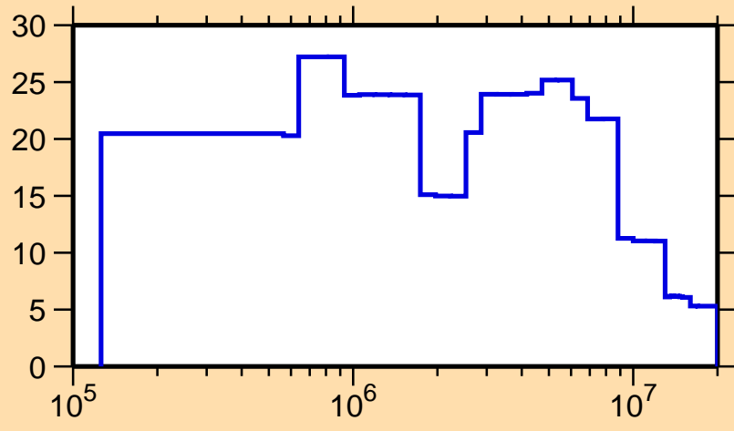
\Delta\sigma/\sigma vs. E for ^{207}\text{Au}(n, el.)
