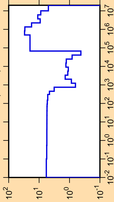
\Delta\sigma/\sigma vs. E for ^{207}\text{Au}(n,\text{tot.})
