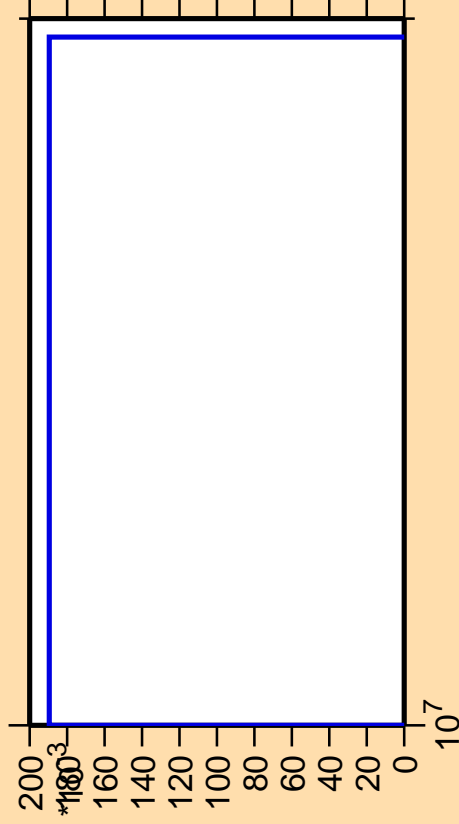
\Delta\sigma/\sigma vs. E for ^{207}\text{Au} (mt 11)
