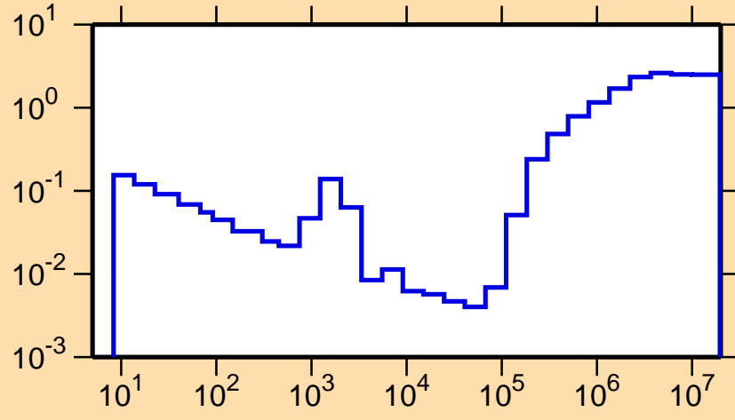
\sigma vs. E for ^{207}\text{Au}(n,\text{nonel.})
