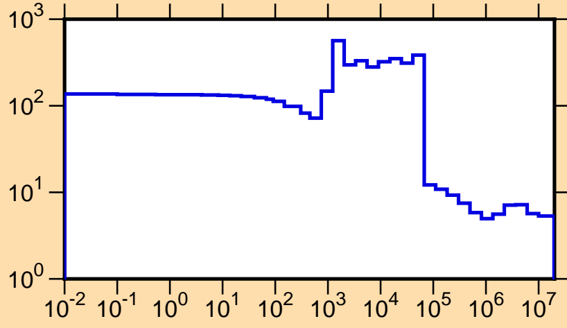
\sigma vs. E for ^{207}\text{Au}(n,\text{tot.})
