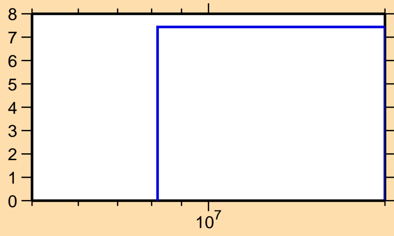
\Delta\sigma/\sigma vs. E for ^{207}\text{Au}(n,\text{el.})
