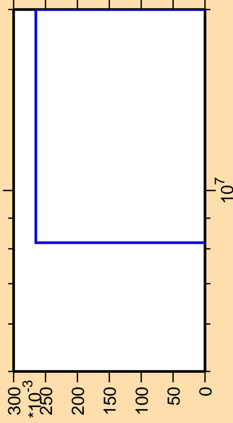
\Delta\sigma/\sigma vs. E for ^{207}\text{Au}(\text{mt } 11)
