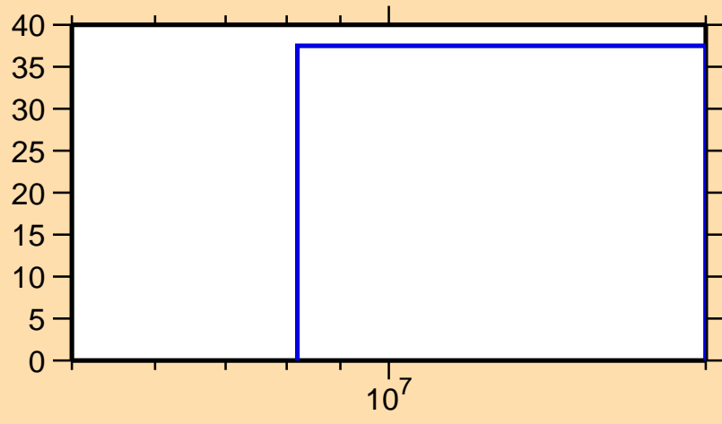
\Delta\sigma/\sigma vs. E for ^{207}\text{Au}(n,\gamma)
