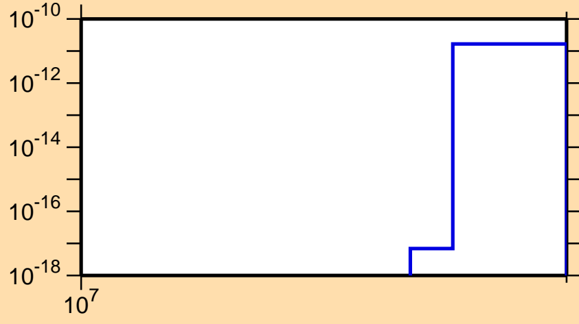
\sigma vs. E for ^{208}\text{Au} (mt 11)
