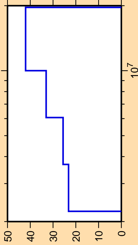
\Delta\sigma/\sigma vs. E for ^{208}\text{Au}(n,n\text{cont.})
