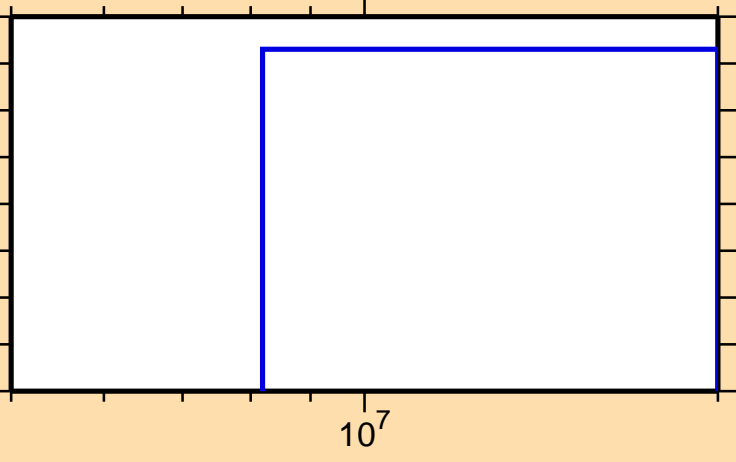
\sigma vs. E for ^{208}\text{Au}(n,d)
