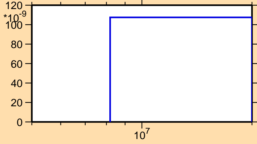
\sigma vs. E for ^{208}\text{Au}(n,nd)
