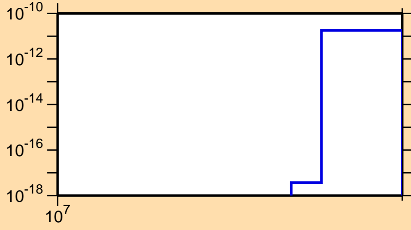
\sigma vs. E for ^{209}\text{Au} (mt 11)
