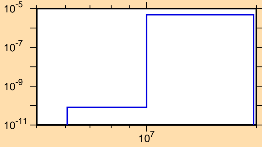
\sigma vs. E for ^{209}\text{Au}(n,\alpha)
