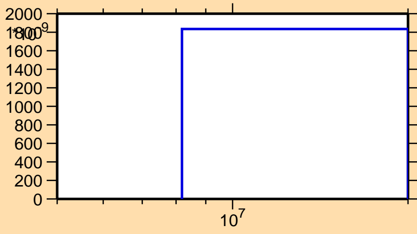
\sigma vs. E for ^{209}\text{Au}(n,np)
