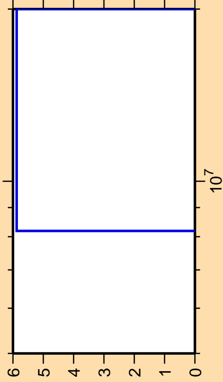
\Delta\sigma/\sigma vs. E for ^{209}\text{Au}(n,3n\alpha)
