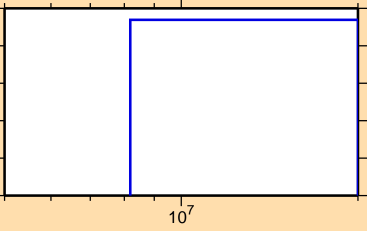
\sigma vs. E for ^{209}\text{Au}(n,\text{nd})
