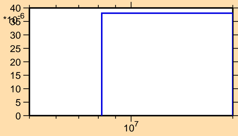
\sigma vs. E for ^{209}\text{Au}(n,p)
