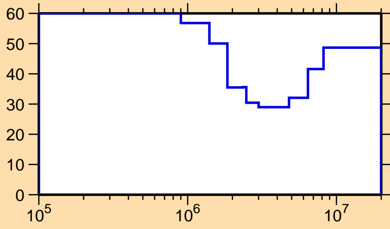
\Delta\sigma/\sigma vs. E for ^{209}\text{Au}(n,n\text{cont.})
