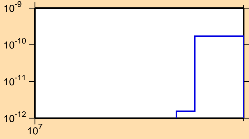
\sigma vs. E for ^{210}\text{Au}(n,3n\alpha)
