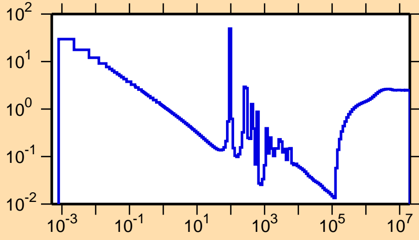
\sigma vs. E for ^{210}\text{Au}(n,\text{nonel.})
