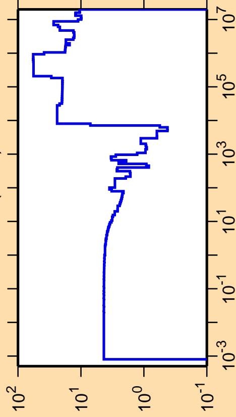
\Delta\sigma/\sigma vs. E for ^{210}\text{Au}(n,\text{el.})
