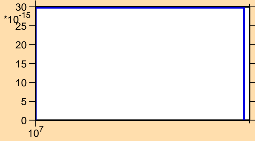
\sigma vs. E for ^{210}\text{Au} (mt 11)
