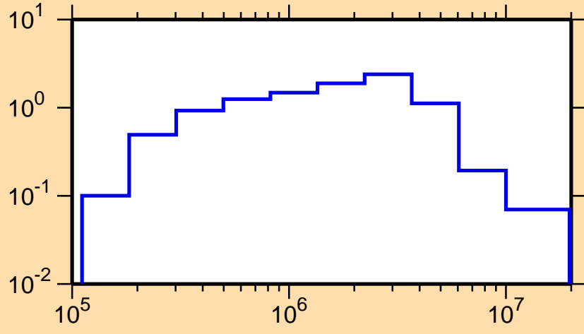
\sigma vs. E for ^{210}\text{Au}(n,\text{inel.})
