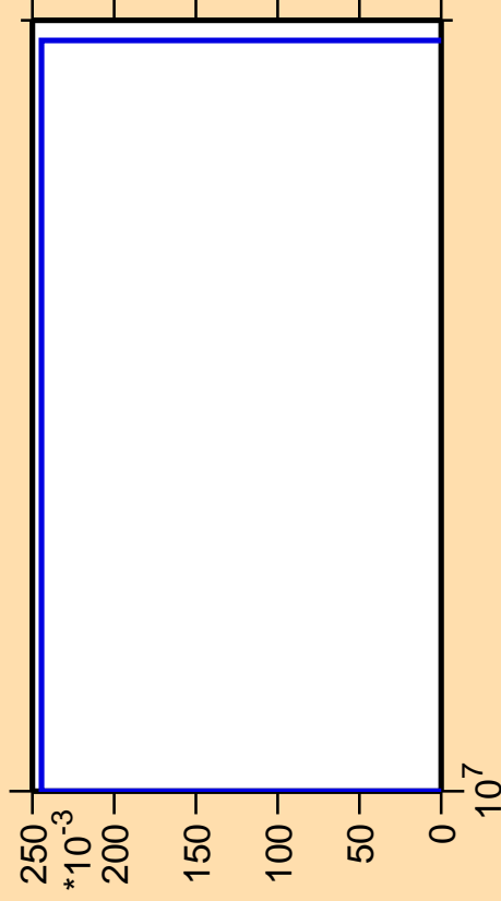
\Delta\sigma/\sigma vs. E for ^{210}\text{Au} (mt 11)
