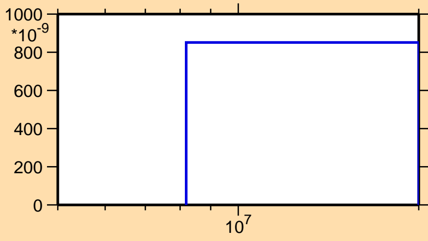
\sigma vs. E for ^{210}\text{Au}(n,n\alpha)
