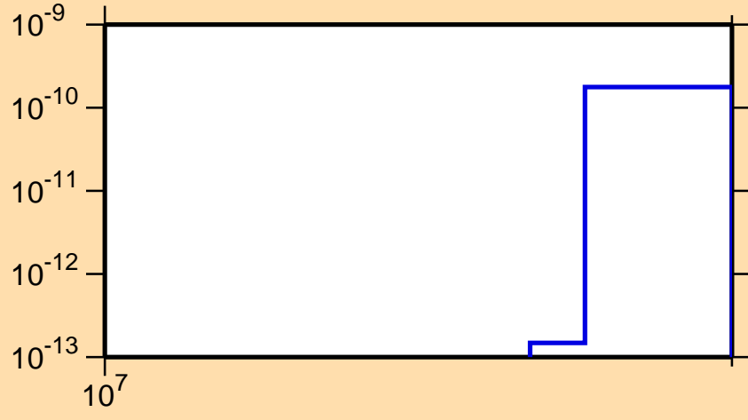
\sigma vs. E for ^{116}\text{Ba}(n,2n\alpha)
