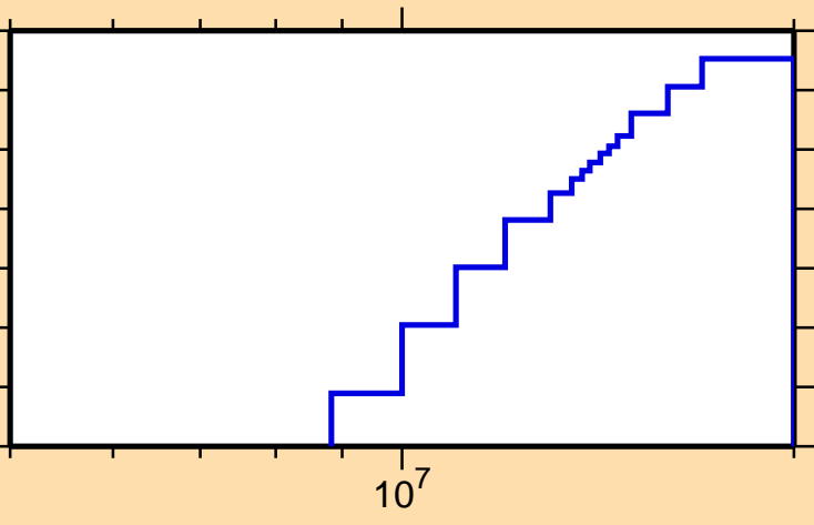
\sigma vs. E for ^{117}\text{Ba}(\text{mt117})
