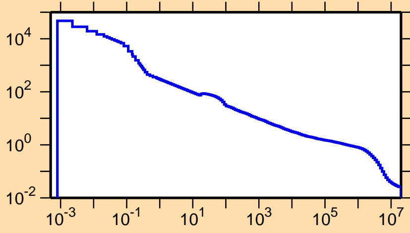
\sigma vs. E for ^{117}\text{Ba}(n,p)
