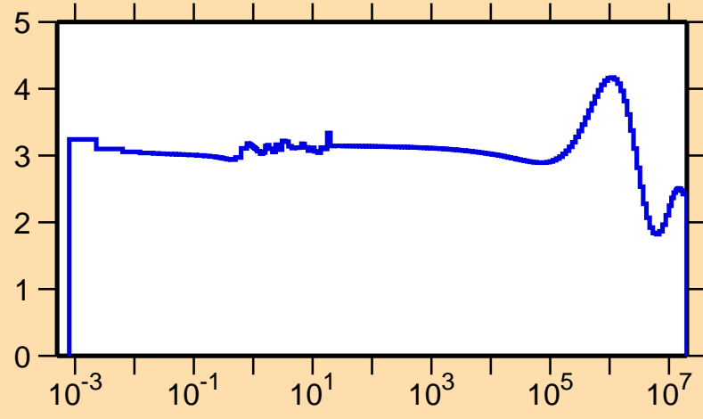
\sigma vs. E for ^{117}\text{Ba}(n,\text{el.})
