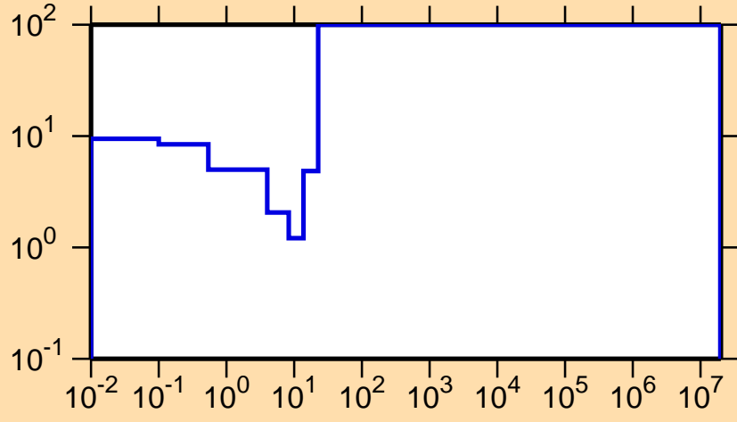
\Delta\sigma/\sigma vs. E for ^{117}\text{Ba}(n,\gamma)
