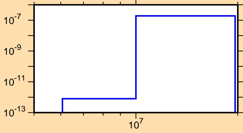
\sigma vs. E for ^{117}\text{Ba}(\text{mt117})
