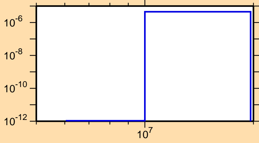
\sigma vs. E for ^{117}\text{Ba}(\text{mt } 45)
