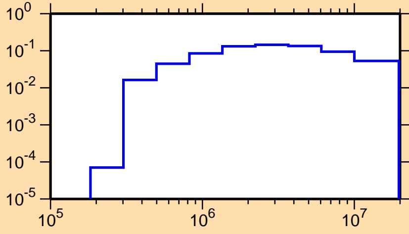
\sigma vs. E for ^{117}\text{Ba}(n,n_1)
