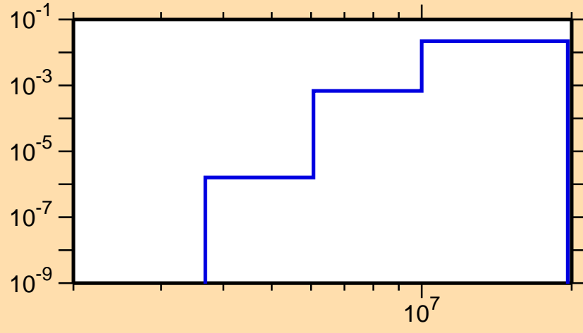
\sigma vs. E for ^{117}\text{Ba}(n,d)
