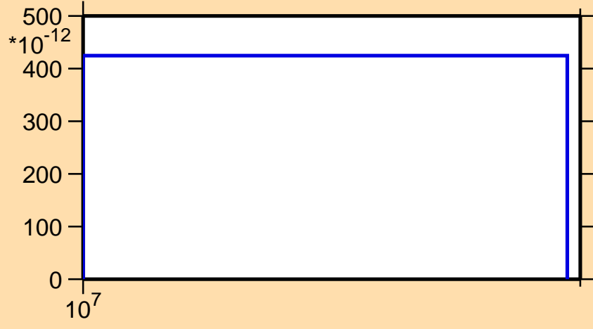
\sigma vs. E for ^{117}\text{Ba}(n,2n\alpha)
