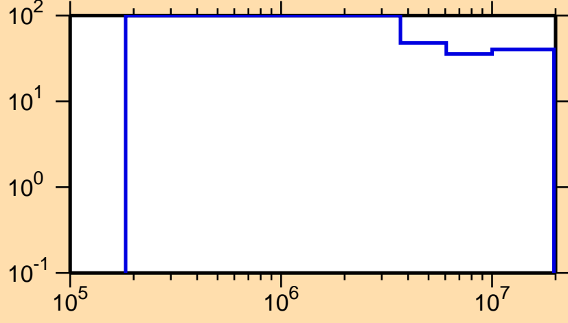
\Delta\sigma/\sigma vs. E for ^{117}\text{Ba}(n,n\text{cont.})
