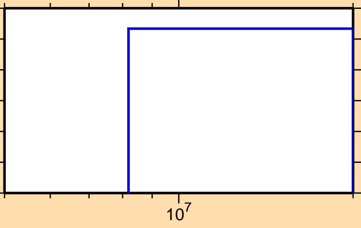
\sigma vs. E for ^{117}\text{Ba}(n,2np)
