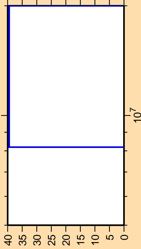
\Delta\sigma/\sigma vs. E for ^{117}\text{Ba}(n,n\text{cont.})
