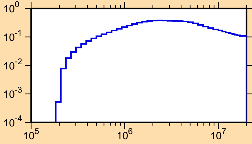
\sigma vs. E for ^{118}\text{Ba}(n,n_1)
