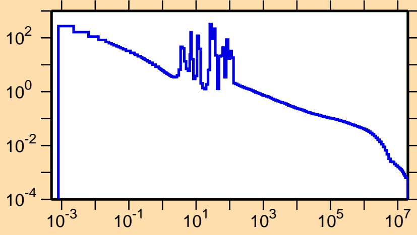
\sigma vs. E for ^{118}\text{Ba}(n,\gamma)
