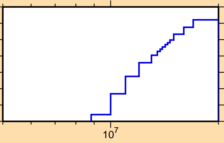
\sigma vs. E for ^{118}\text{Ba}(\text{mt117})
