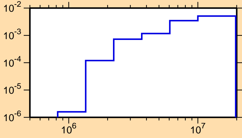
\sigma vs. E for ^{118}\text{Ba}(n,n\text{cont.})
