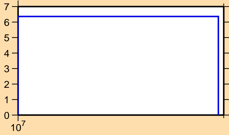
\Delta\sigma/\sigma vs. E for ^{118}\text{Ba}(n,\text{tot.})
