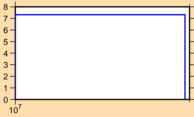
\Delta\sigma/\sigma vs. E for ^{118}\text{Ba}(n,\text{el.})
