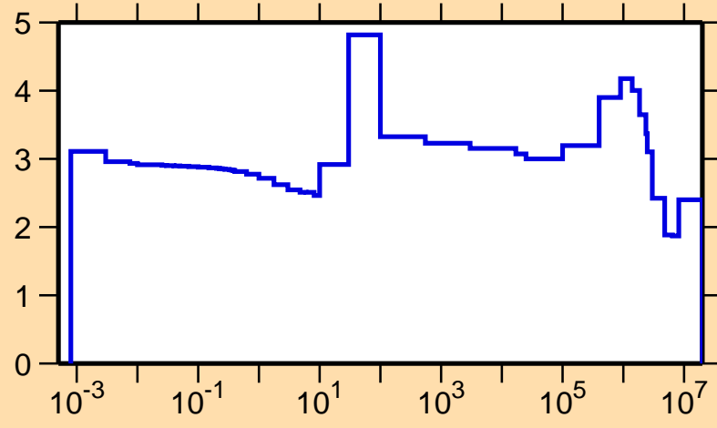
\sigma vs. E for ^{118}\text{Ba}(n,\text{el.})
