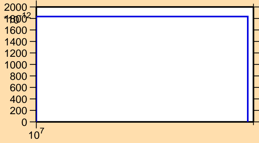
\sigma vs. E for ^{119}\text{Ba}(n,2n\alpha)
