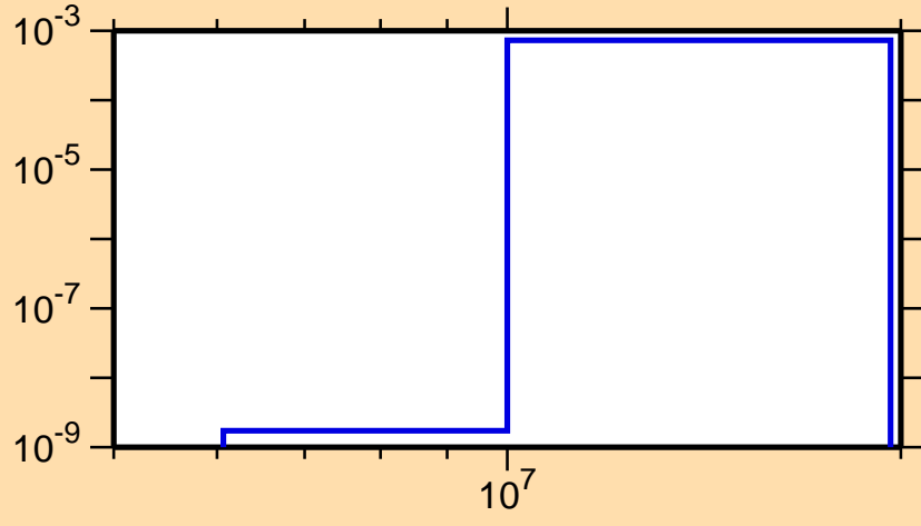
\sigma vs. E for ^{119}\text{Ba}(n,\text{pd})
