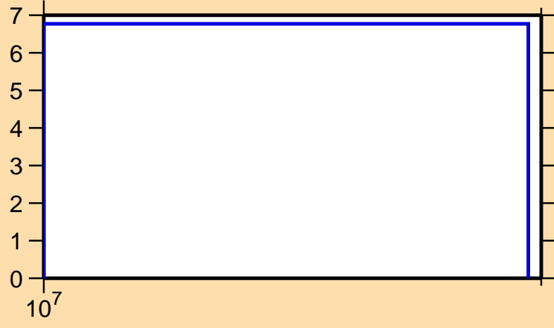
\Delta\sigma/\sigma vs. E for ^{119}\text{Ba}(n,\text{el.})
