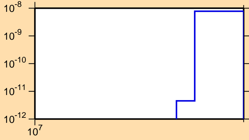
\sigma vs. E for ^{120}\text{Ba}(n,\text{nd})
