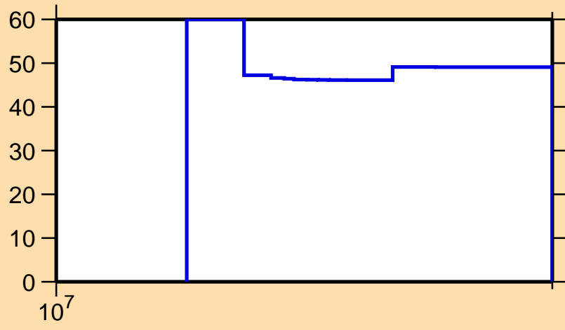
\Delta\sigma/\sigma vs. E for ^{120}\text{Ba}(n,2n)
