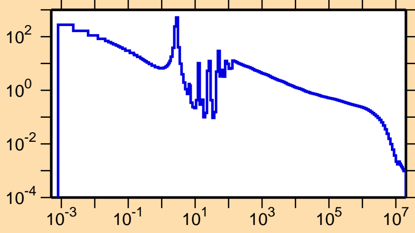
\sigma vs. E for ^{120}\text{Ba}(n,\gamma)
