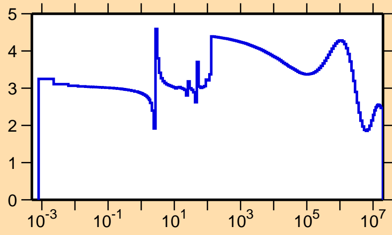
\sigma vs. E for ^{120}\text{Ba}(n,\text{el.})
