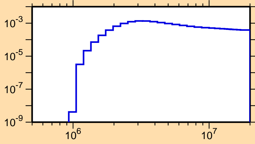
\sigma vs. E for ^{120}\text{Ba}(n,n_3)
