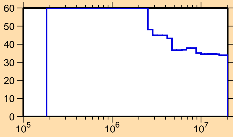
\Delta\sigma/\sigma vs. E for ^{120}\text{Ba}(n,\text{inel.})
