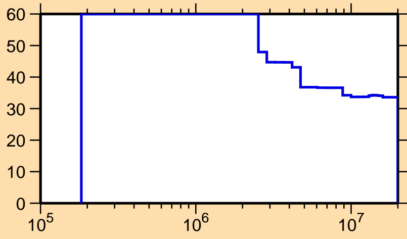
\Delta\sigma/\sigma vs. E for ^{120}\text{Ba}(n,n_1)
