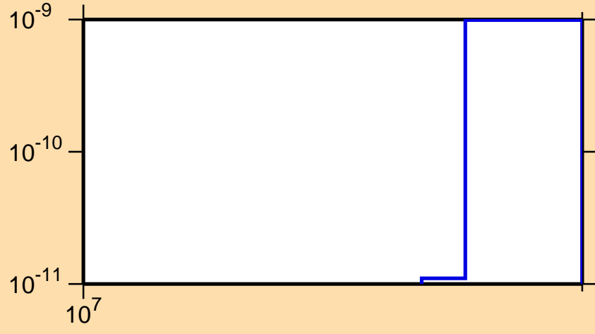
\sigma vs. E for ^{120}\text{Ba} (mt 34)
