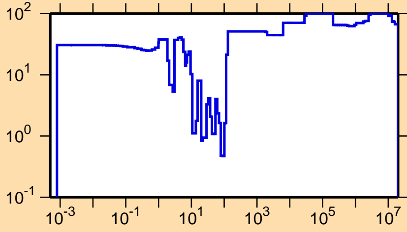
\Delta\sigma/\sigma vs. E for ^{120}\text{Ba}(n,\gamma)
