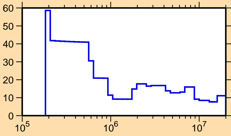
\Delta\sigma/\sigma vs. E for ^{120}\text{Ba}(n,\text{el.})
