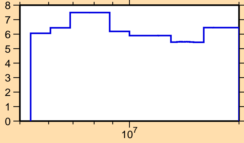
\Delta\sigma/\sigma vs. E for ^{120}\text{Ba}(n,\text{nonel.})
