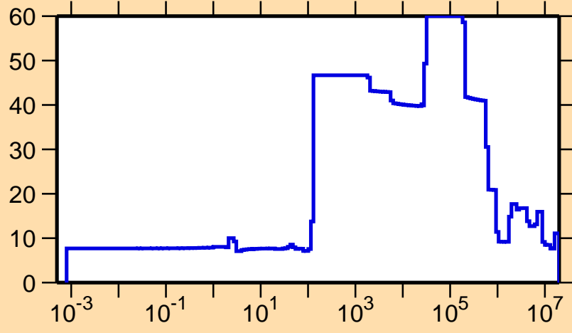
\Delta\sigma/\sigma vs. E for ^{120}\text{Ba}(n,\text{el.})
