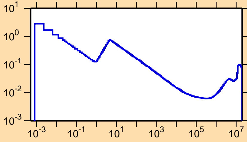
\sigma vs. E for ^{120}\text{Ba}(n,\alpha)
