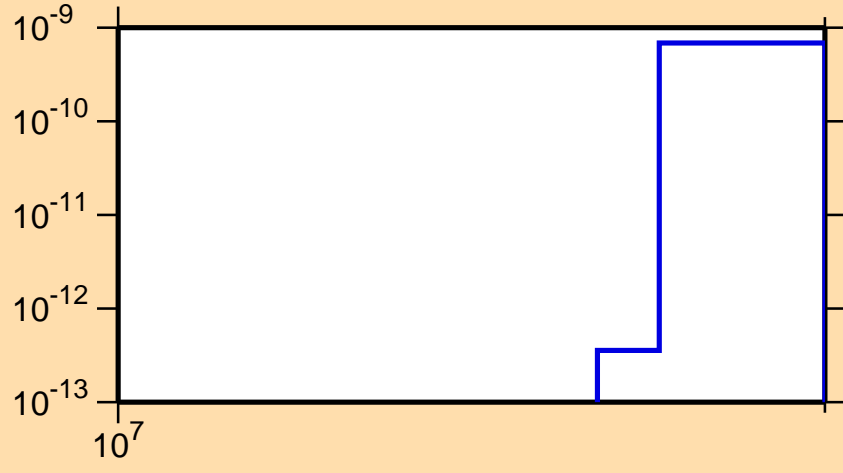
\sigma vs. E for ^{120}\text{Ba}(n,2n\alpha)
