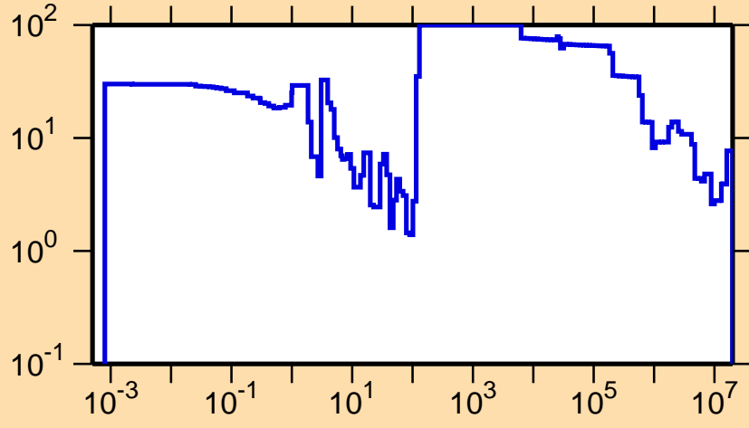
\Delta\sigma/\sigma vs. E for ^{120}\text{Ba}(n,\text{tot.})
