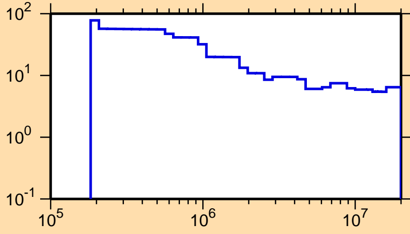
\Delta\sigma/\sigma vs. E for ^{120}\text{Ba}(n,\text{nonel.})
