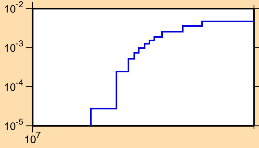
\sigma vs. E for ^{120}\text{Ba}(n,2n)
