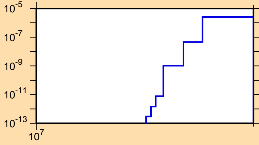
\sigma vs. E for ^{120}\text{Ba}(n,\text{pt})
