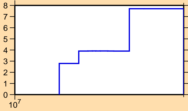
\Delta\sigma/\sigma vs. E for ^{120}\text{Ba}(n,\text{tot.})
