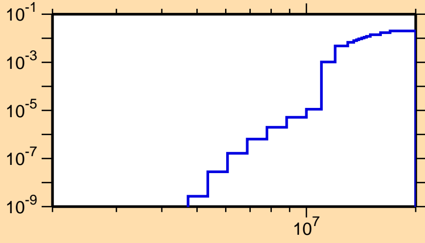
\sigma vs. E for ^{120}\text{Ba}(n,d)
