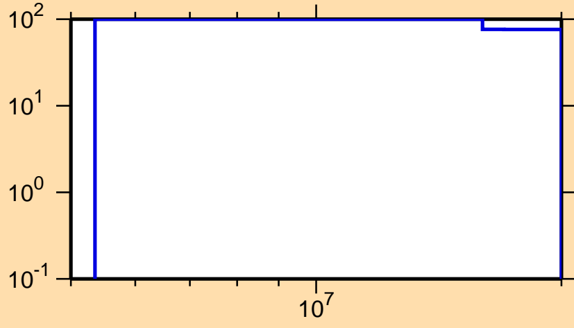
\Delta\sigma/\sigma vs. E for ^{120}\text{Ba}(n,n\text{cont.})
