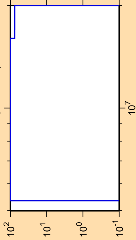
\Delta\sigma/\sigma vs. E for ^{120}\text{Ba}(n,\text{ncont.})
