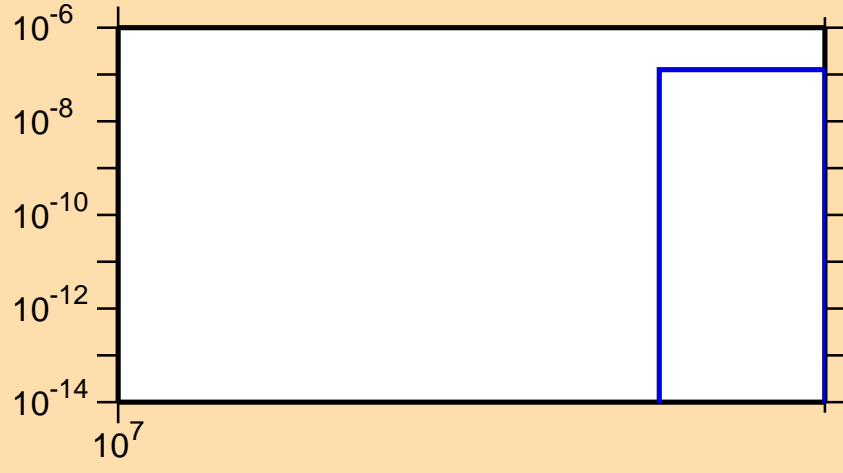
\sigma vs. E for ^{120}\text{Ba}(n,2np)
