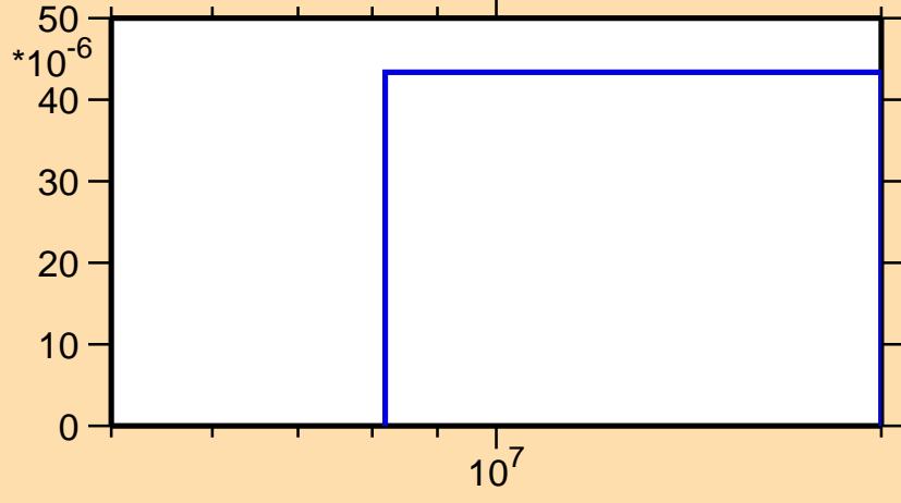
\sigma vs. E for ^{120}\text{Ba}(n,t)
