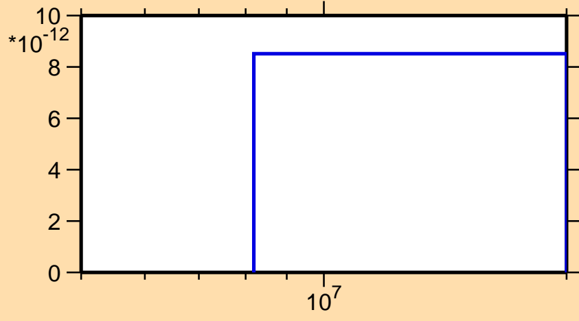
\sigma vs. E for ^{120}\text{Ba} (mt 34)
