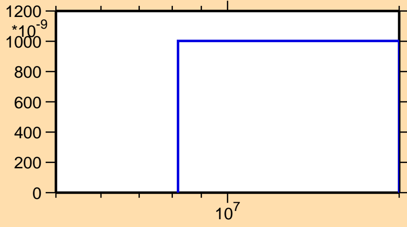
\sigma vs. E for ^{120}\text{Ba} (mt 45)
