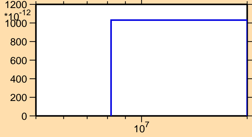
\sigma vs. E for ^{120}\text{Ba}(n,2np)
