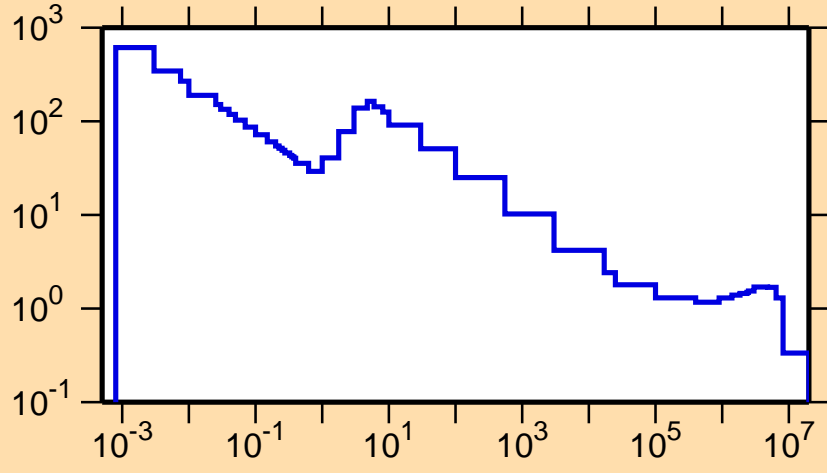
\sigma vs. E for ^{120}\text{Ba}(n,p)
