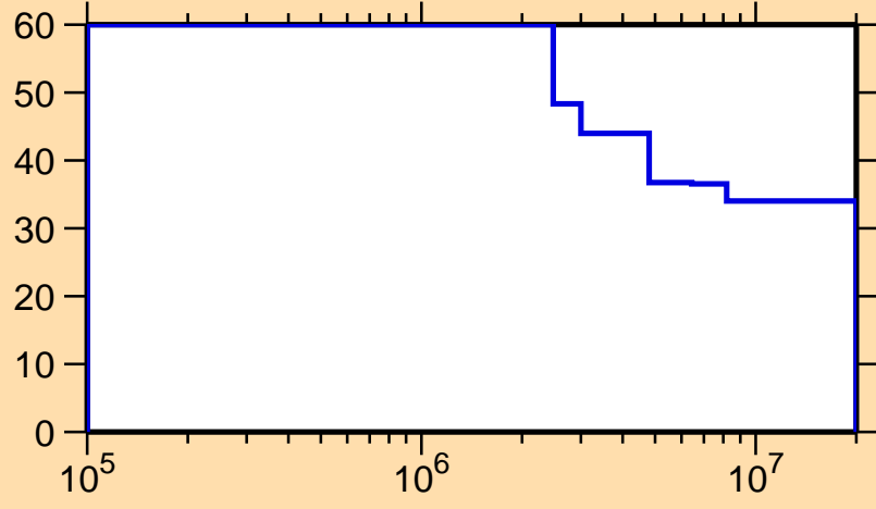
\Delta\sigma/\sigma vs. E for ^{120}\text{Ba}(n,n_1)
