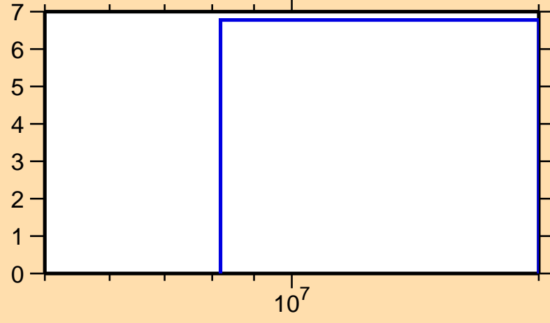
\Delta\sigma/\sigma vs. E for ^{120}\text{Ba}(n,\text{el.})
