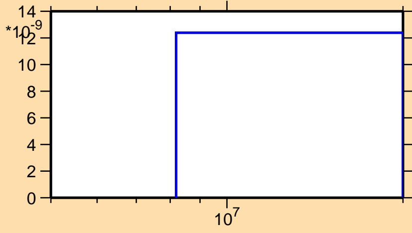
\sigma vs. E for ^{120}\text{Ba}(\text{mt117})
