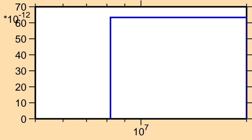
\sigma vs. E for ^{120}\text{Ba}(n,\text{nd})
