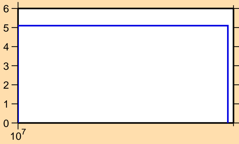
\Delta\sigma/\sigma vs. E for ^{121}\text{Ba}(n,\text{nonel.})
