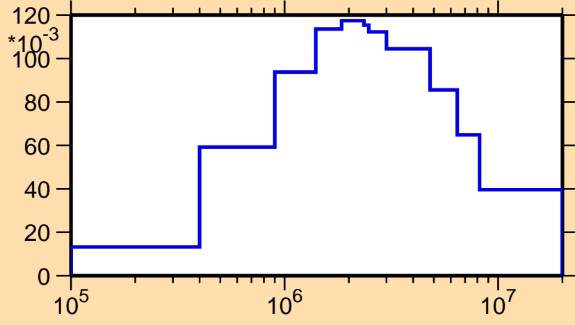
\sigma vs. E for ^{121}\text{Ba}(n,n_3)
