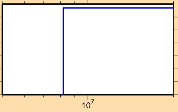
\sigma vs. E for ^{121}\text{Ba} (mt 34)
