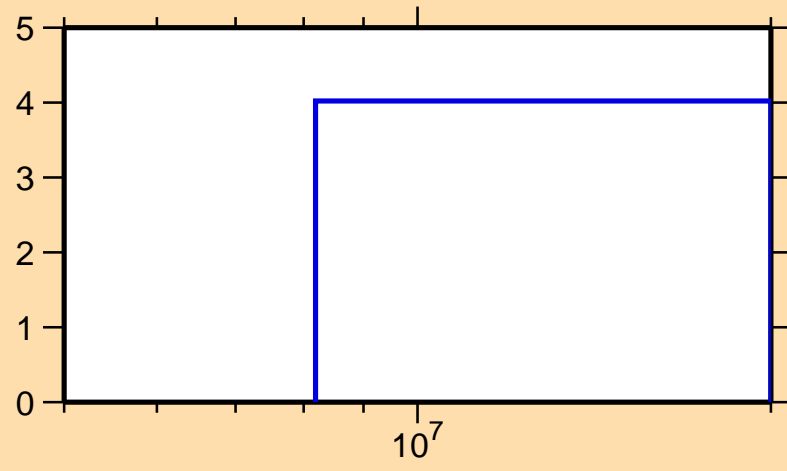
\Delta\sigma/\sigma vs. E for ^{121}\text{Ba}(n,\text{el.})
