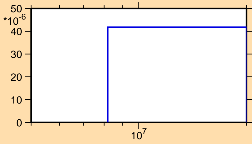
\sigma vs. E for ^{121}\text{Ba}(n,\text{pd})
