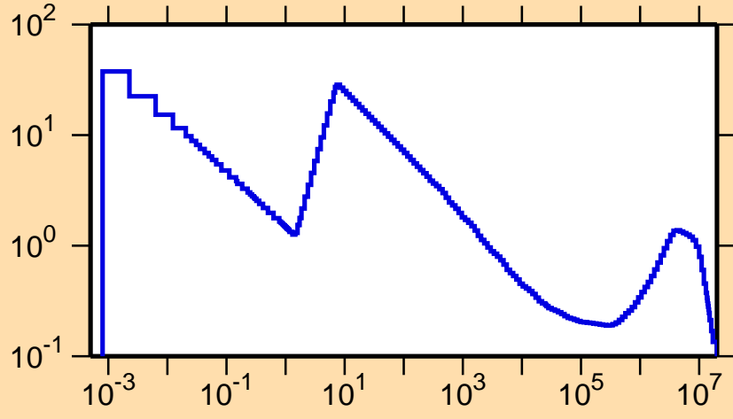
\sigma vs. E for ^{122}\text{Ba}(n,p)
