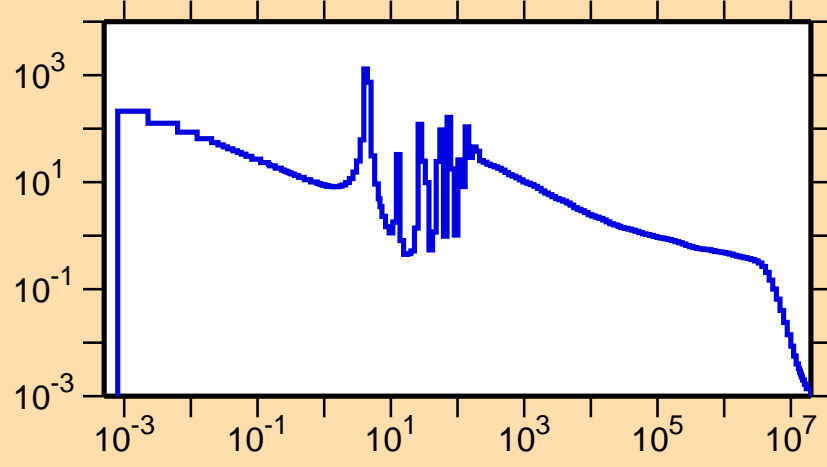
\sigma vs. E for ^{122}\text{Ba}(n,\gamma)
