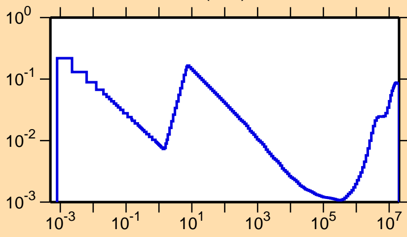
\sigma vs. E for ^{122}\text{Ba}(n,\alpha)
