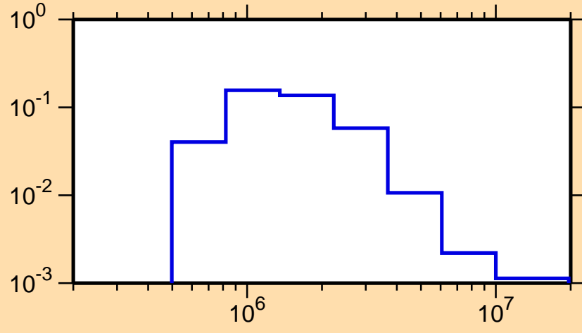
\sigma vs. E for ^{122}\text{Ba}(n,n_3)
