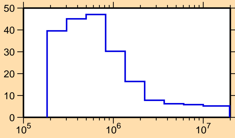
\Delta\sigma/\sigma vs. E for ^{122}\text{Ba}(n,\text{nonel.})
