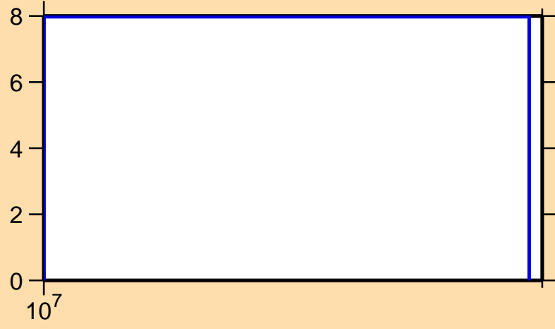
\Delta\sigma/\sigma vs. E for ^{122}\text{Ba}(n,\text{el.})
