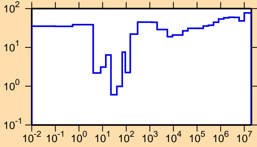
\Delta\sigma/\sigma vs. E for ^{122}\text{Ba}(n,\gamma)
