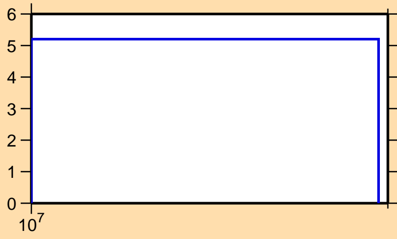
\Delta\sigma/\sigma vs. E for ^{122}\text{Ba}(n,\text{nonel.})
