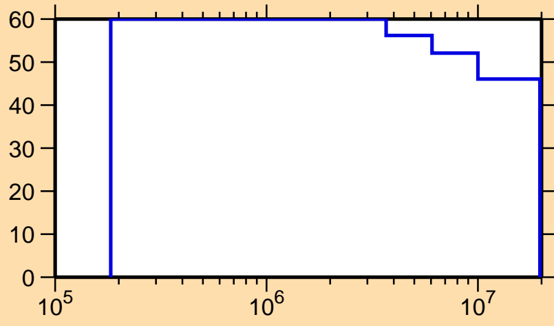
\Delta\sigma/\sigma vs. E for ^{122}\text{Ba}(n,n_1)
