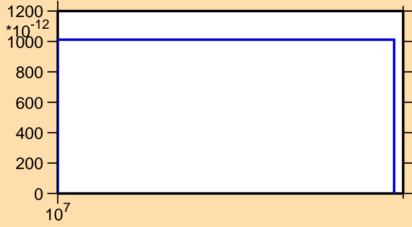
\sigma vs. E for ^{122}\text{Ba}(n,2np)
