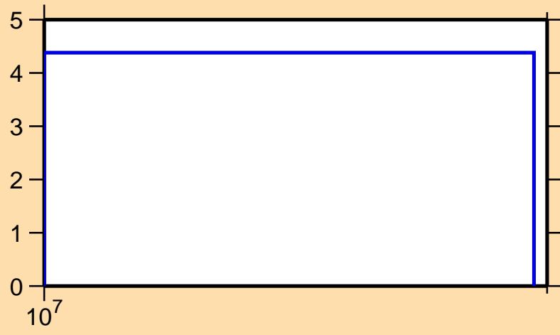
\Delta\sigma/\sigma vs. E for ^{122}\text{Ba}(n,\text{tot.})
