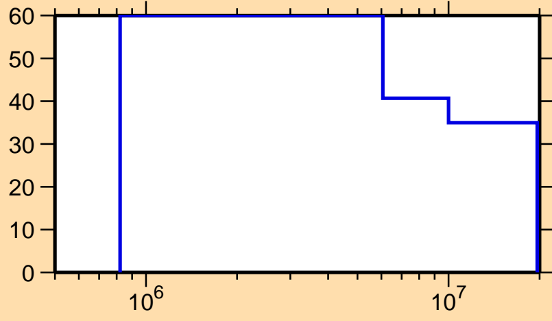
\Delta\sigma/\sigma vs. E for ^{122}\text{Ba}(n,n\text{cont.})
