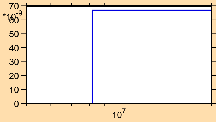
\sigma vs. E for ^{122}\text{Ba} (mt 45)
