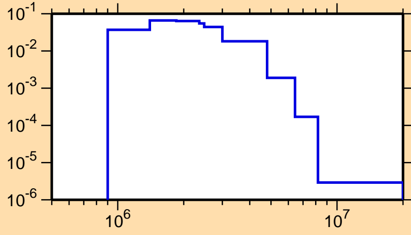
\sigma vs. E for ^{122}\text{Ba}(n,n_4)
