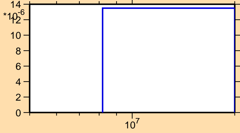
\sigma vs. E for ^{122}\text{Ba}(n,pd)
