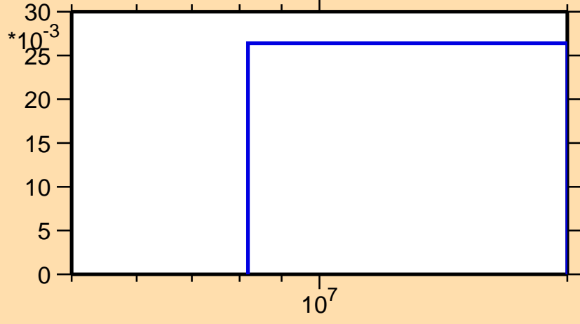
\sigma vs. E for ^{122}\text{Ba}(n,2n)
