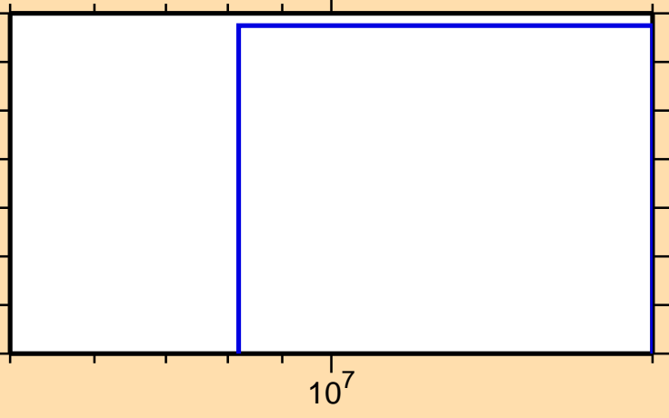
\sigma vs. E for ^{122}\text{Ba}(n,pd)
