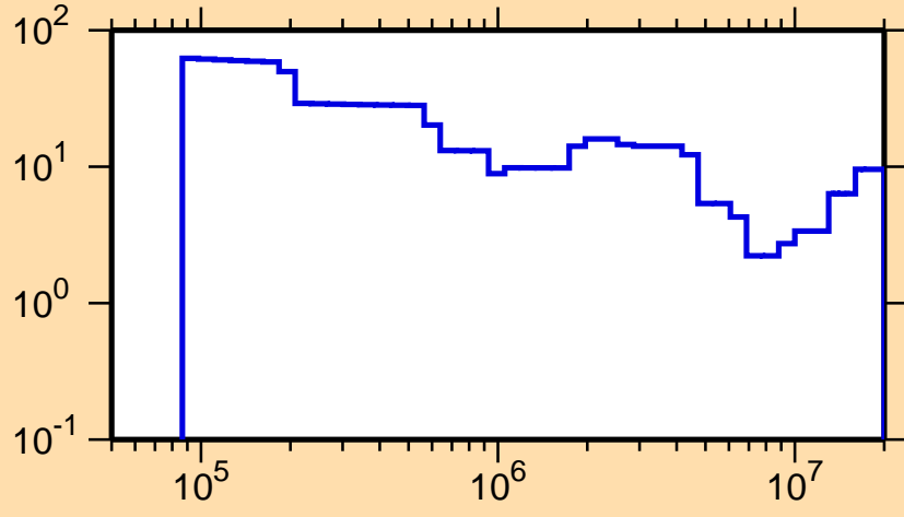
\Delta\sigma/\sigma vs. E for ^{123}\text{Ba}(n,\text{tot.})
