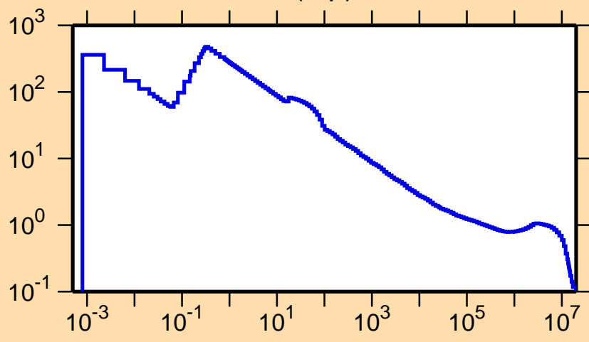
\sigma vs. E for ^{123}\text{Ba}(n,p)
