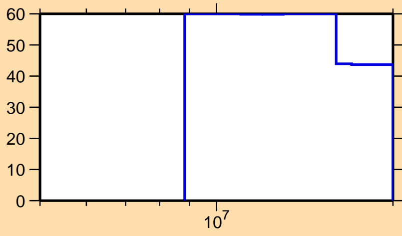
\Delta\sigma/\sigma vs. E for ^{123}\text{Ba}(n,2n)
