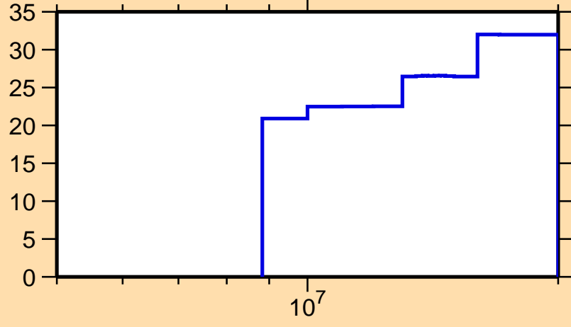
\Delta\sigma/\sigma vs. E for ^{123}\text{Ba}(n,\text{inel.})
