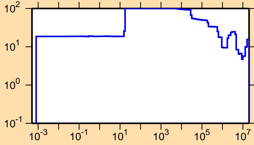
\Delta\sigma/\sigma vs. E for ^{123}\text{Ba}(n,\text{el.})
