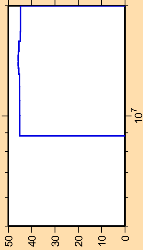
\Delta\sigma/\sigma vs. E for ^{123}\text{Ba}(n,n_1)
