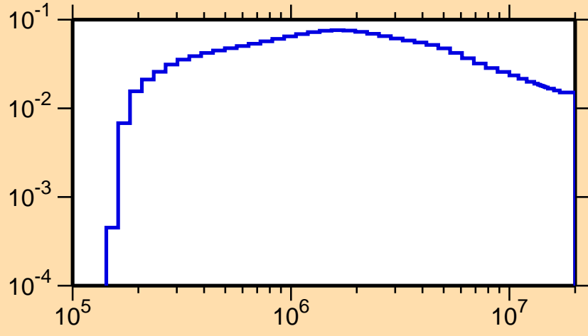
\sigma vs. E for ^{123}\text{Ba}(n,n_3)
