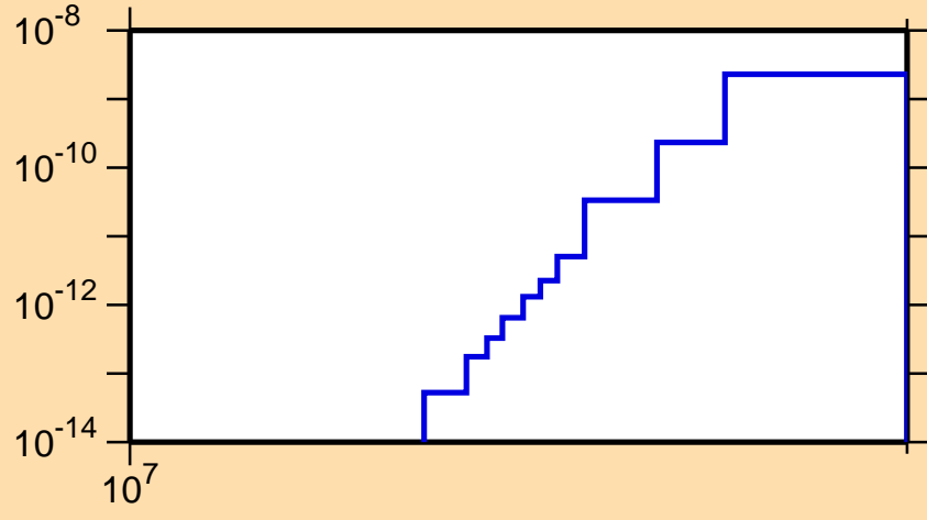
\sigma vs. E for ^{123}\text{Ba}(\text{mt117})
