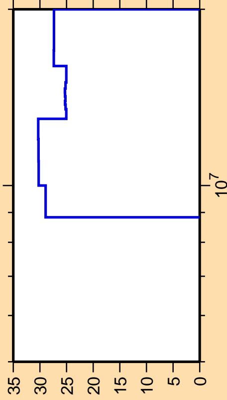
\Delta\sigma/\sigma vs. E for ^{123}\text{Ba}(n,n\text{cont.})
