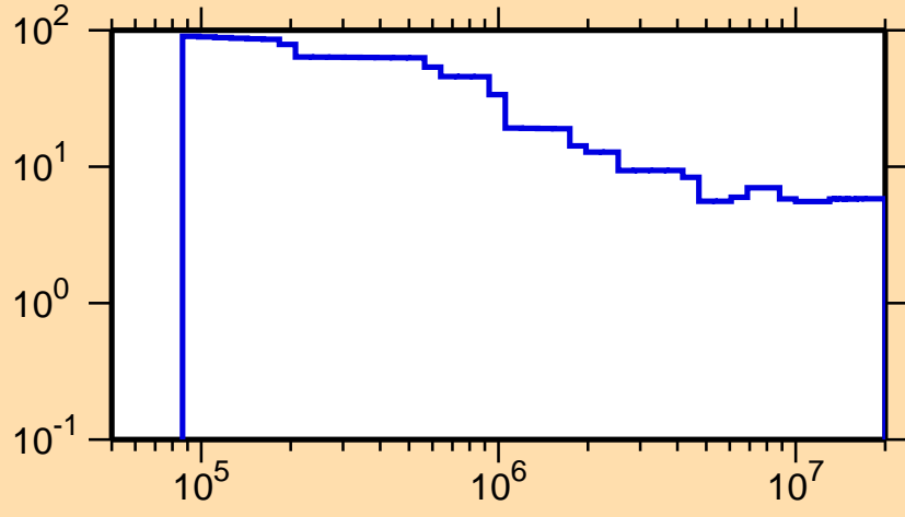
\Delta\sigma/\sigma vs. E for ^{123}\text{Ba}(n,\text{nonel.})
