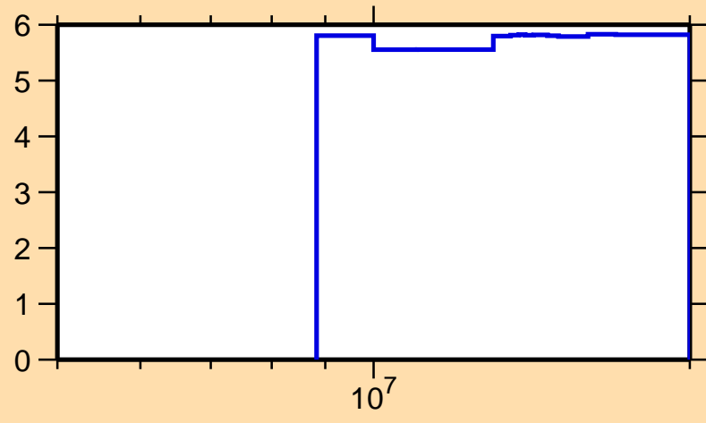
\Delta\sigma/\sigma vs. E for ^{123}\text{Ba}(n,\text{nonel.})
