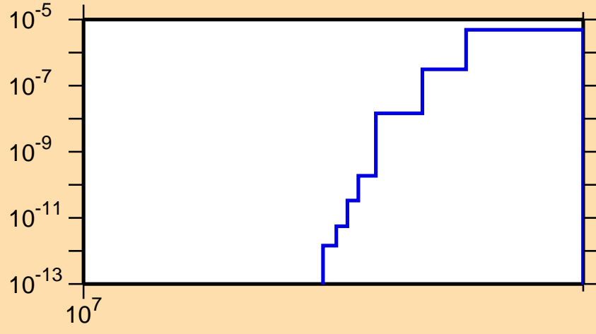
\sigma vs. E for ^{123}\text{Ba}(n,\text{nd})
