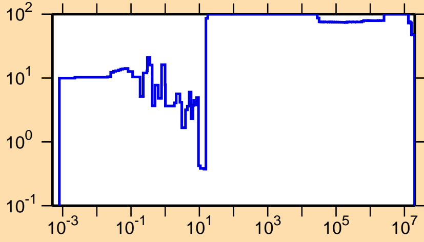
\Delta\sigma/\sigma vs. E for ^{123}\text{Ba}(n,\gamma)
