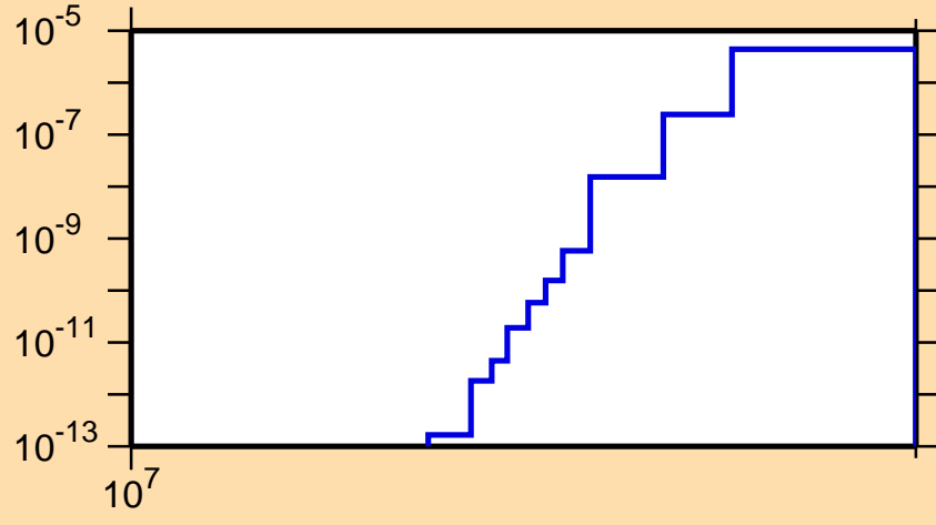
\sigma vs. E for ^{123}\text{Ba}(n,\text{pt})
