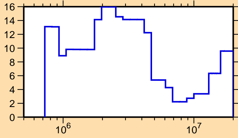
\Delta\sigma/\sigma vs. E for ^{123}\text{Ba}(n,\text{tot.})
