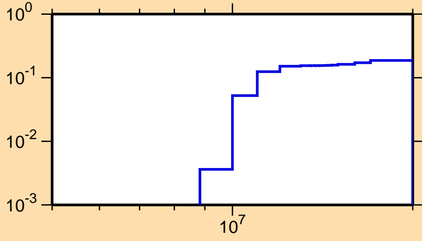
\sigma vs. E for ^{123}\text{Ba}(n,2n)
