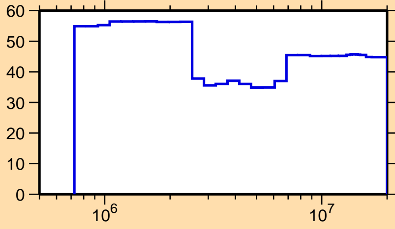
\Delta\sigma/\sigma vs. E for ^{123}\text{Ba}(n,n_1)
