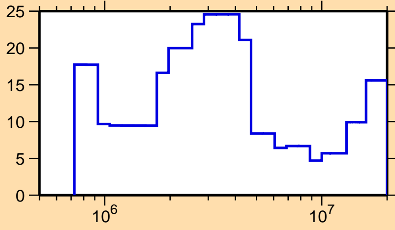
\Delta\sigma/\sigma vs. E for ^{123}\text{Ba}(n,\text{el.})
