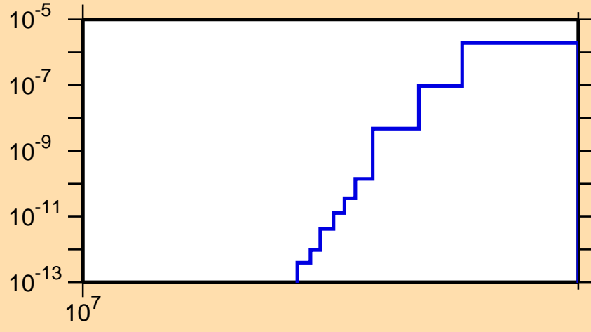
\sigma vs. E for ^{123}\text{Ba}(n,2n\alpha)
