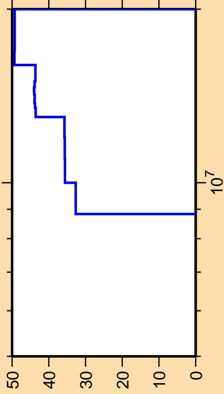
\Delta\sigma/\sigma vs. E for ^{123}\text{Ba}(n,p)
