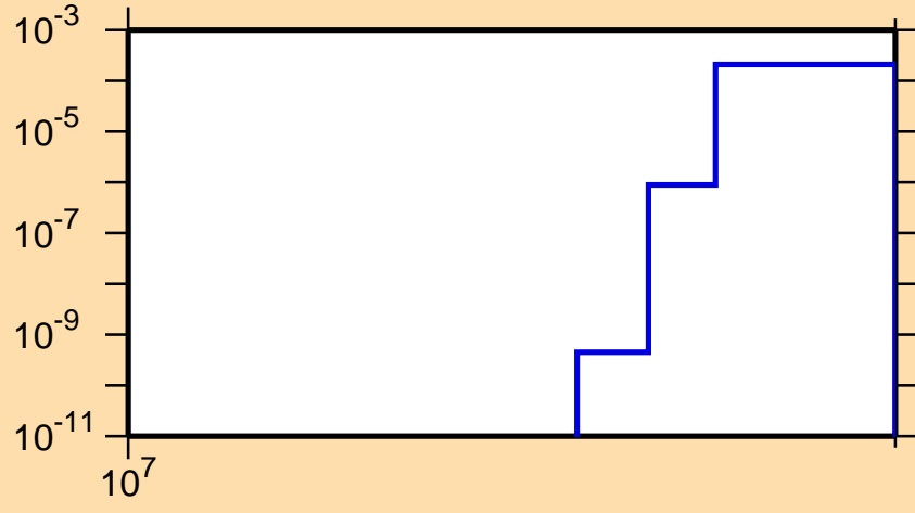
\sigma vs. E for ^{123}\text{Ba}(n,2np)
