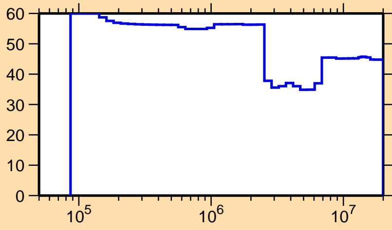
\Delta\sigma/\sigma vs. E for ^{123}\text{Ba}(n,n_1)
