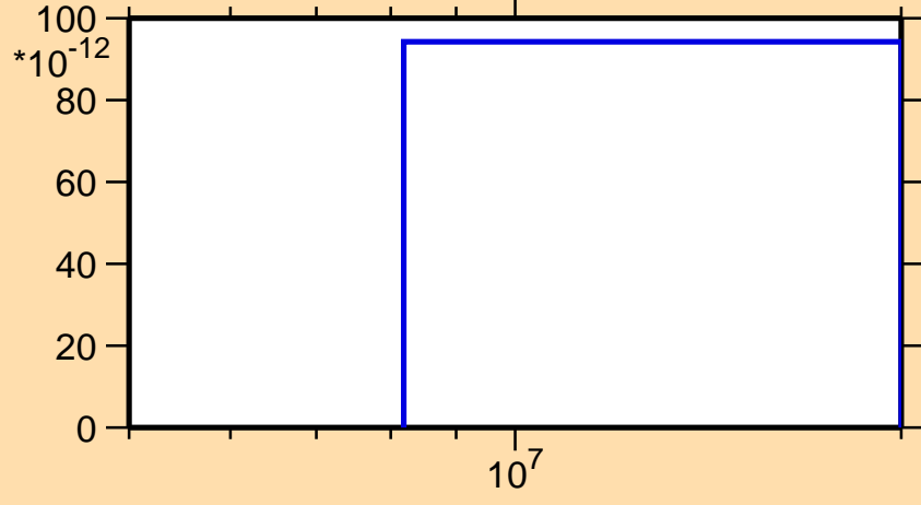
\sigma vs. E for ^{123}\text{Ba}(\text{mt } 34)
