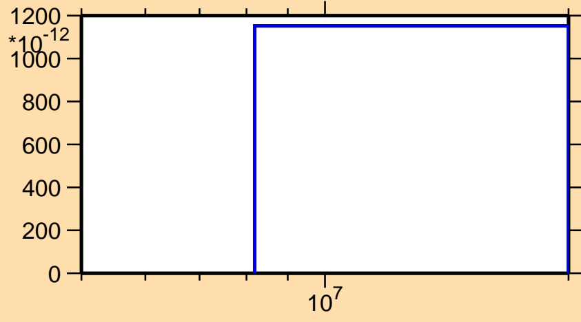
\sigma vs. E for ^{123}\text{Ba} (mt 45)
