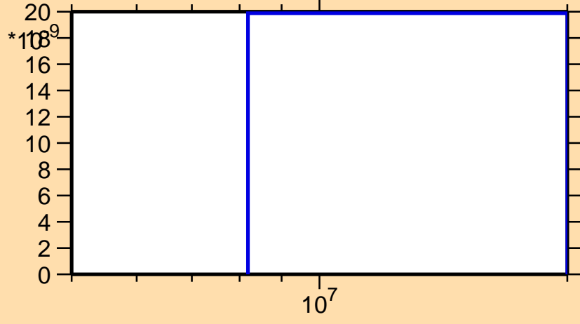
\sigma vs. E for ^{123}\text{Ba}(n,2n\alpha)
