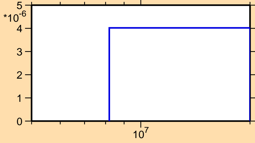
\sigma vs. E for ^{123}\text{Ba}(n,\text{pd})
