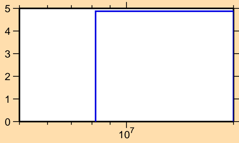
\Delta\sigma/\sigma vs. E for ^{123}\text{Ba}(n,\text{tot.})
