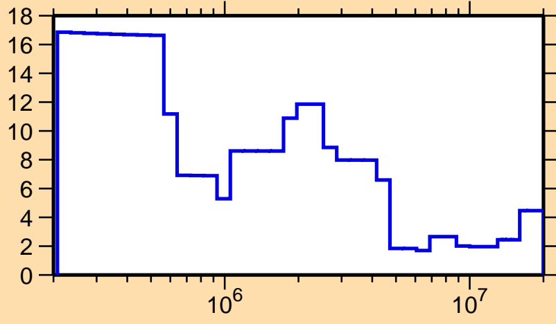
\Delta\sigma/\sigma vs. E for ^{124}\text{Ba}(n,\text{tot.})
