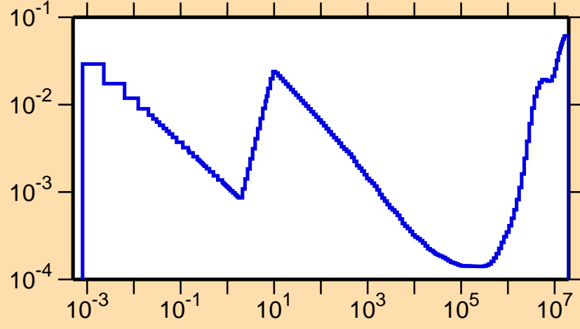
\sigma vs. E for ^{124}\text{Ba}(n,\alpha)
