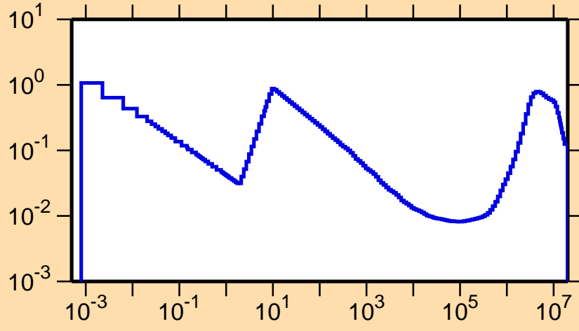
\sigma vs. E for ^{124}\text{Ba}(n,p)
