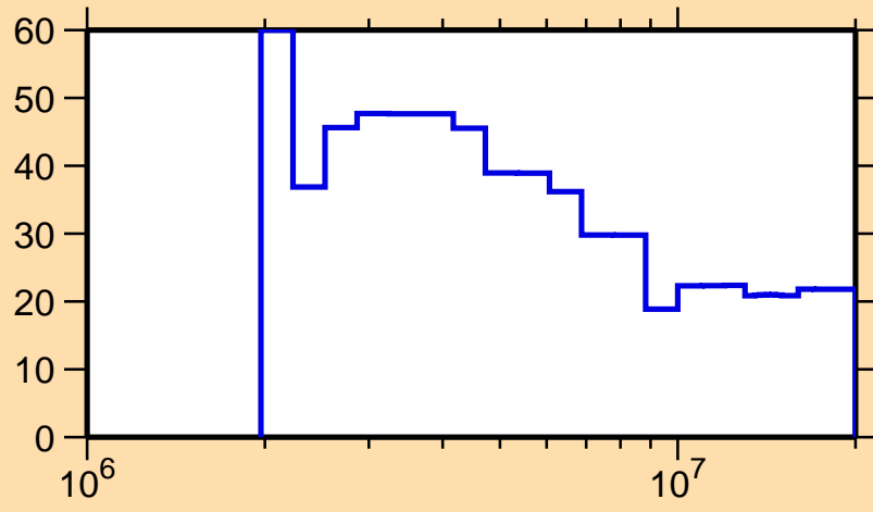
\Delta\sigma/\sigma vs. E for ^{124}\text{Ba}(n,n\text{cont.})
