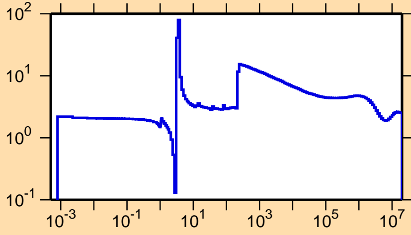
\sigma vs. E for ^{124}\text{Ba}(n,\text{el.})
