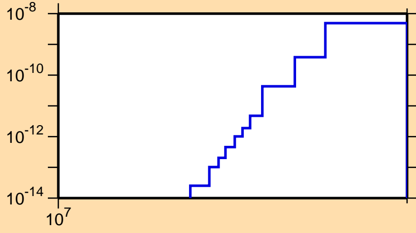
\sigma vs. E for ^{124}\text{Ba}(\text{mt117})
