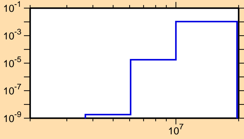
\sigma vs. E for ^{124}\text{Ba}(n,n\alpha)
