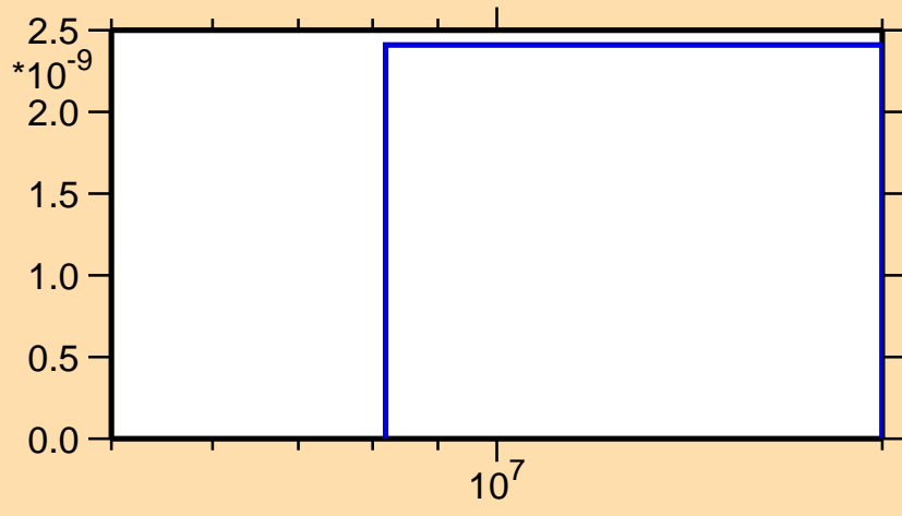
\sigma vs. E for ^{124}\text{Ba}(\text{mt } 45)
