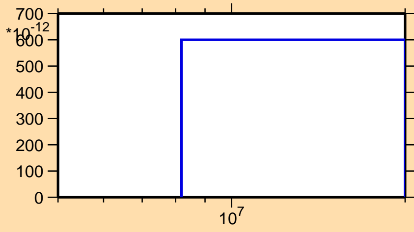
\sigma vs. E for ^{124}\text{Ba}(n,\text{nd})
