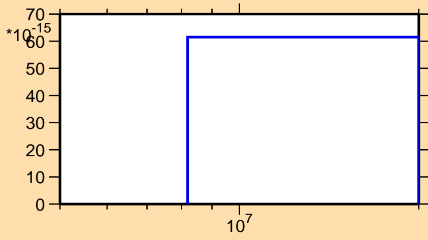
\sigma vs. E for ^{124}\text{Ba}(\text{mt } 34)
