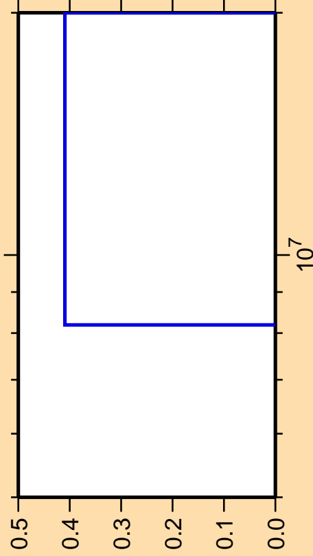
\Delta\sigma/\sigma vs. E for ^{124}\text{Ba}(\text{mt } 34)
