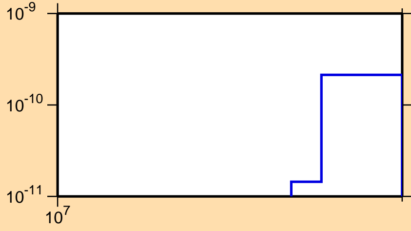
\sigma vs. E for ^{125}\text{Ba}(\text{mt117})
