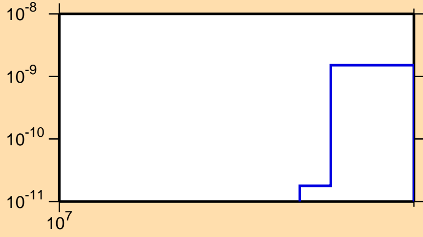
\sigma vs. E for ^{125}\text{Ba} (mt 34)
