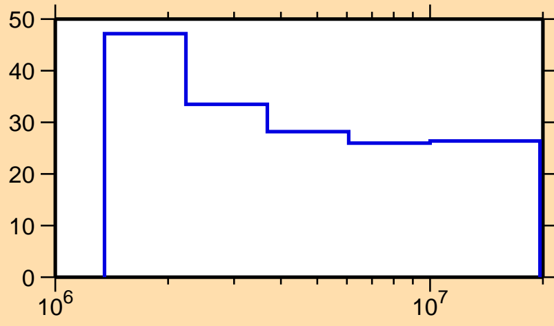
\Delta\sigma/\sigma vs. E for ^{125}\text{Ba}(n,n_1)
