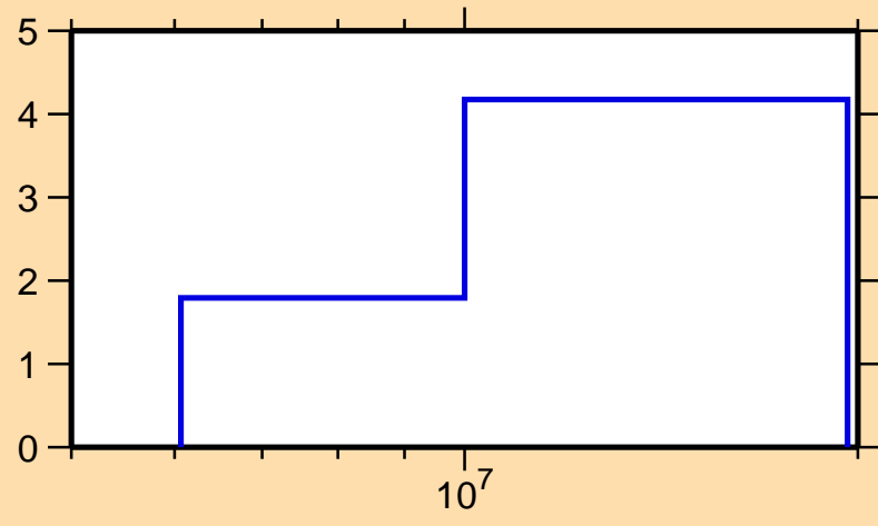
\Delta\sigma/\sigma vs. E for ^{125}\text{Ba}(n,\text{tot.})
