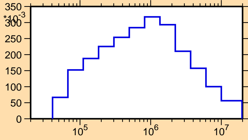
\sigma vs. E for ^{125}\text{Ba}(n,n_1)
