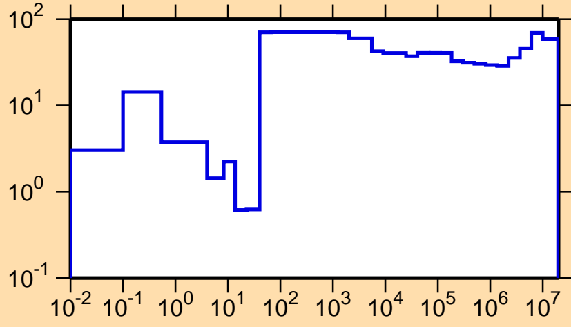
\Delta\sigma/\sigma vs. E for ^{125}\text{Ba}(n,\gamma)
