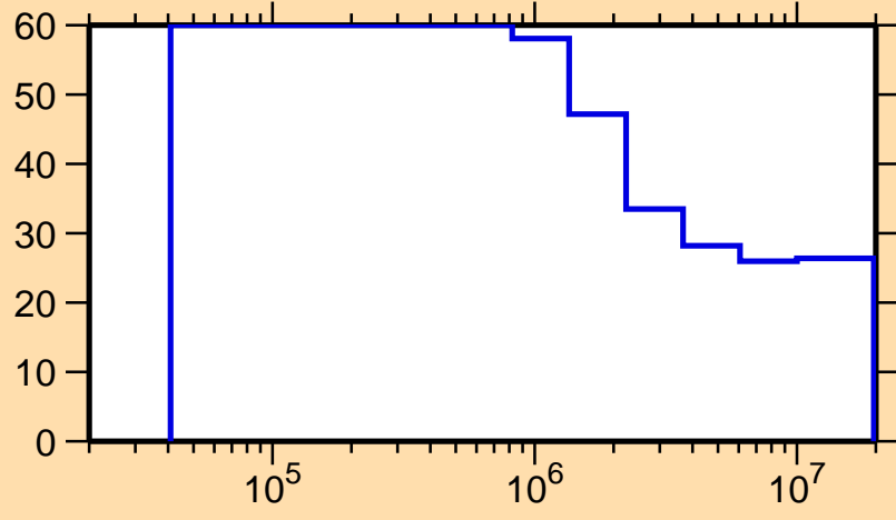
\Delta\sigma/\sigma vs. E for ^{125}\text{Ba}(n,n_1)
