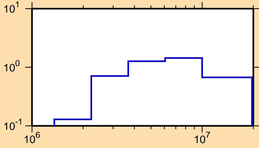
\sigma vs. E for ^{125}\text{Ba}(n,n\text{cont.})
