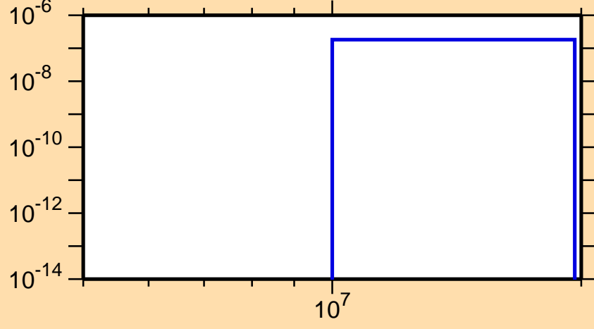
\sigma vs. E for ^{125}\text{Ba}(n,pd)
