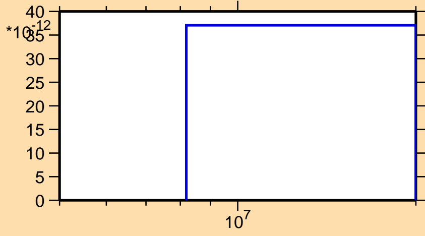
\sigma vs. E for ^{125}\text{Ba} (mt 45)
