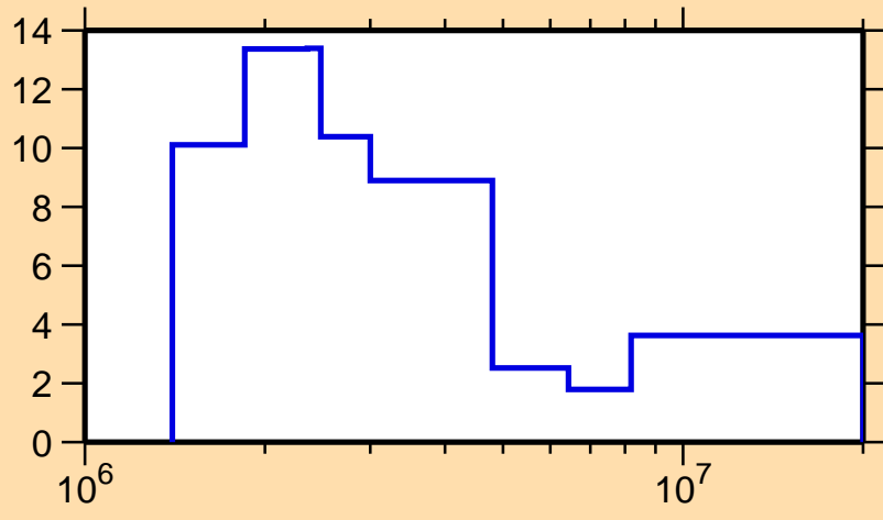
\Delta\sigma/\sigma vs. E for ^{125}\text{Ba}(n,\text{tot.})
