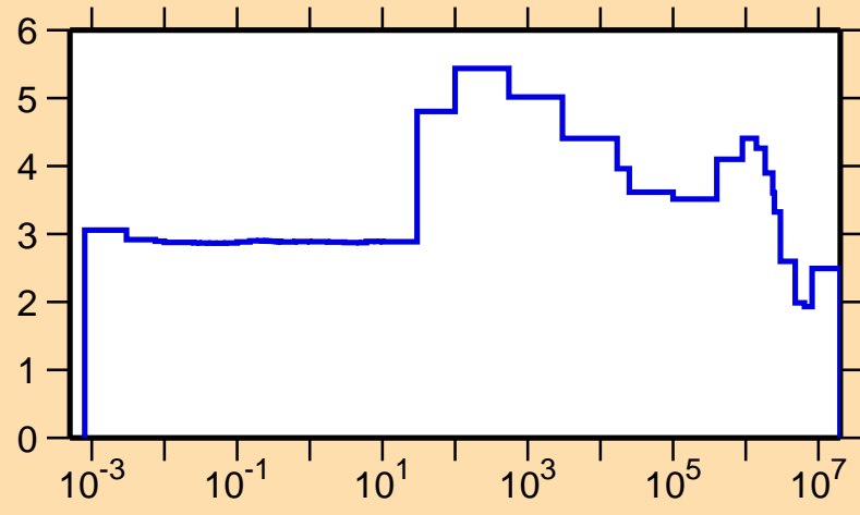
\sigma vs. E for ^{125}\text{Ba}(n,\text{el.})
