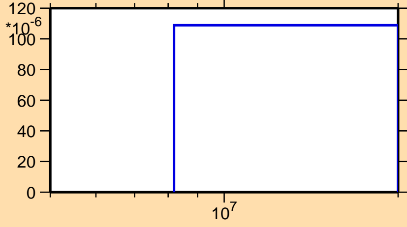
\sigma vs. E for ^{125}\text{Ba}(n,t)
