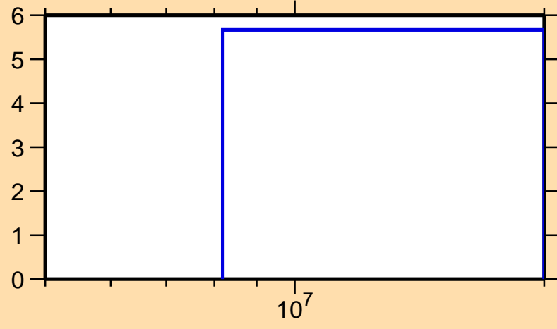
\Delta\sigma/\sigma vs. E for ^{125}\text{Ba}(n,\text{el.})
