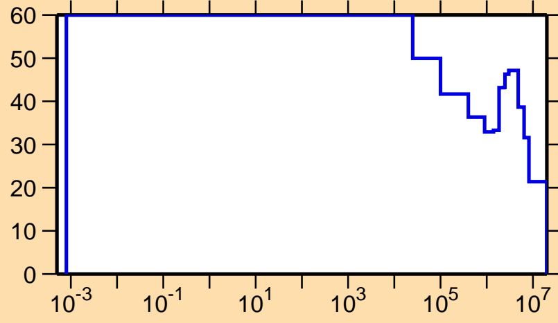
\Delta\sigma/\sigma vs. E for ^{125}\text{Ba}(n,p)
