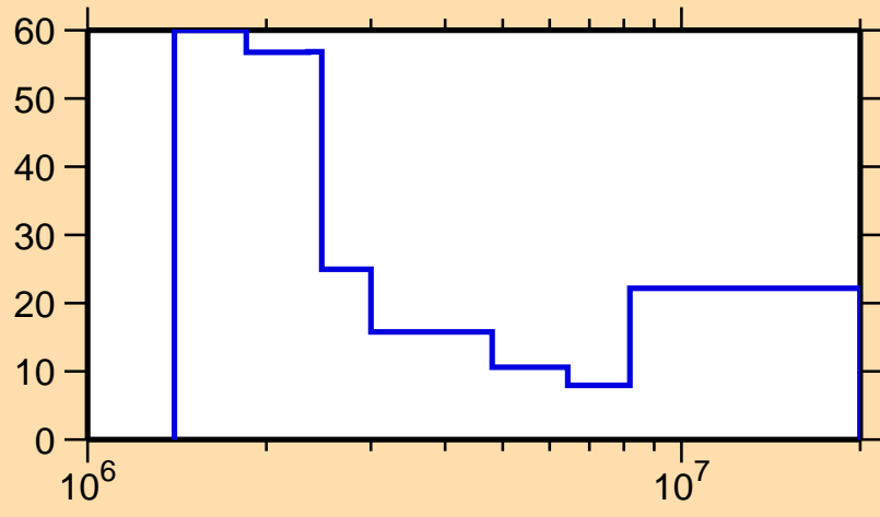
\Delta\sigma/\sigma vs. E for ^{125}\text{Ba}(n,n\text{cont.})
