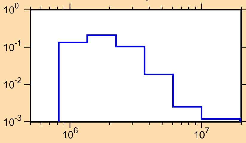
\sigma vs. E for ^{126}\text{Ba}(n,n_3)
