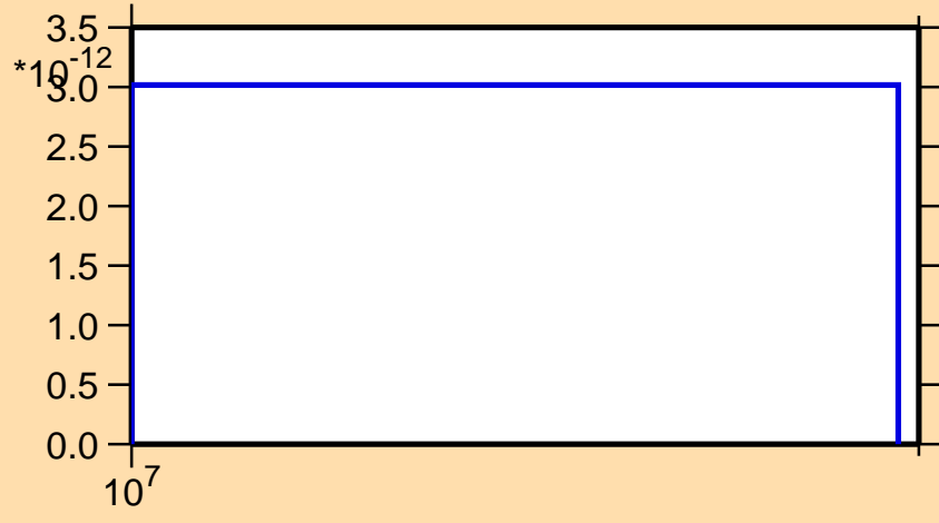
\sigma vs. E for ^{126}\text{Ba}(\text{mt117})
