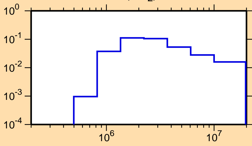
\sigma vs. E for ^{126}\text{Ba}(n,n_2)
