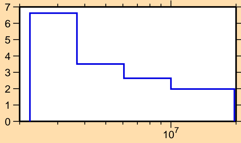
\Delta\sigma/\sigma vs. E for ^{126}\text{Ba}(n,\text{tot.})
