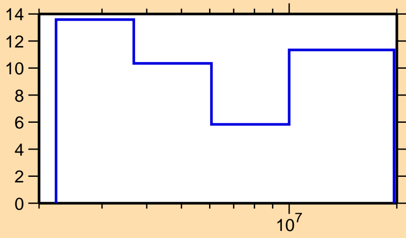
\Delta\sigma/\sigma vs. E for ^{126}\text{Ba}(n,n\text{cont.})
