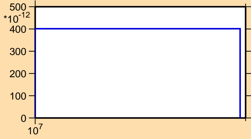
\sigma vs. E for ^{126}\text{Ba}(n,2np)
