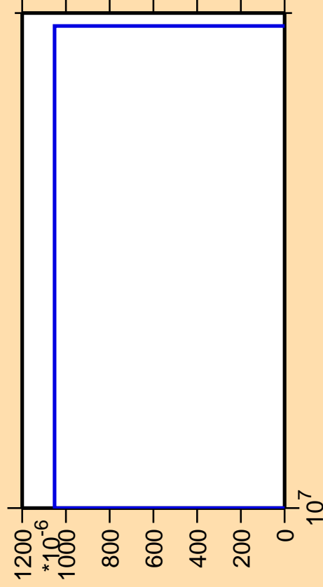
\Delta\sigma/\sigma vs. E for ^{126}\text{Ba}(n,nt)
