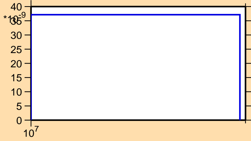
\sigma vs. E for ^{126}\text{Ba}(n,\text{pd})
