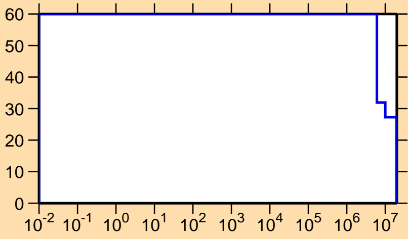
\Delta\sigma/\sigma vs. E for ^{126}\text{Ba}(n,p)
