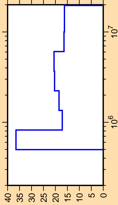
\Delta\sigma/\sigma vs. E for ^{126}\text{Ba}(n,n_2)
