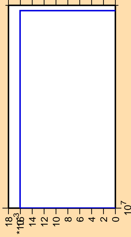
\Delta\sigma/\sigma vs. E for ^{126}\text{Ba} (mt 34)
