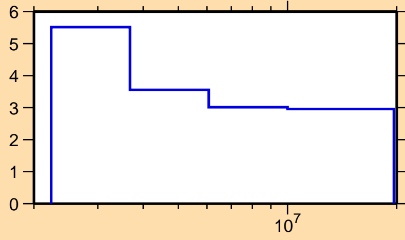
\Delta\sigma/\sigma vs. E for ^{126}\text{Ba}(n,\text{nonel.})
