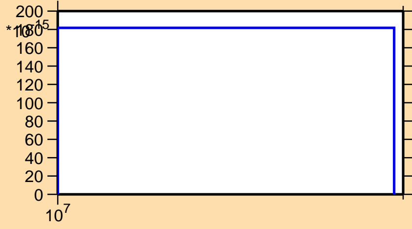
\sigma vs. E for ^{126}\text{Ba}(n,\text{pt})
