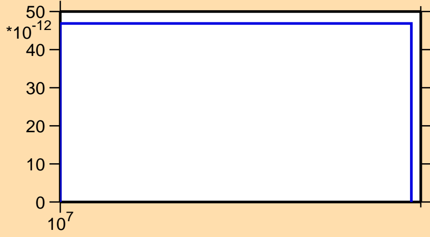
\sigma vs. E for ^{126}\text{Ba} (mt 45)
