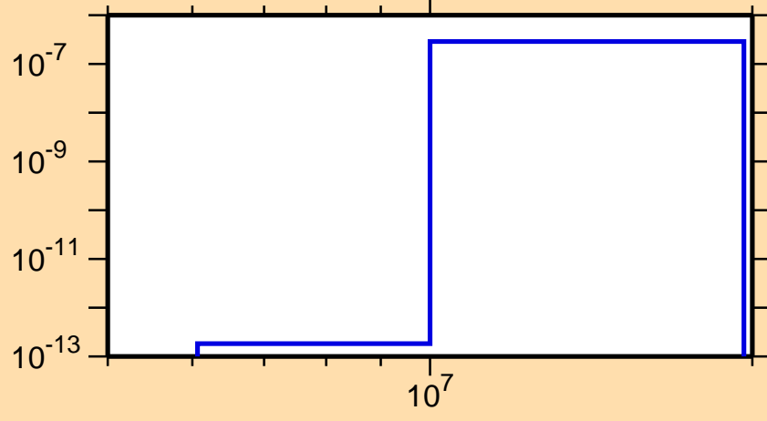
\sigma vs. E for ^{126}\text{Ba}(n,\text{He}3)
