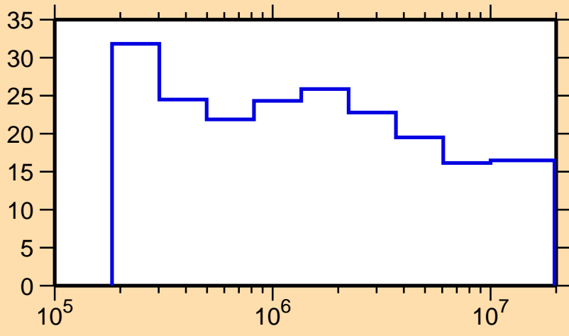
\Delta\sigma/\sigma vs. E for ^{126}\text{Ba}(n,n_1)
