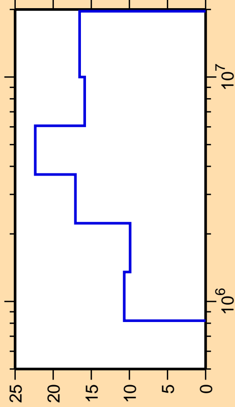
\Delta\sigma/\sigma vs. E for ^{126}\text{Ba}(n,n_3)
