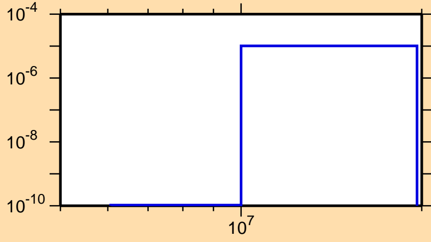
\sigma vs. E for ^{126}\text{Ba}(n,p\alpha)
