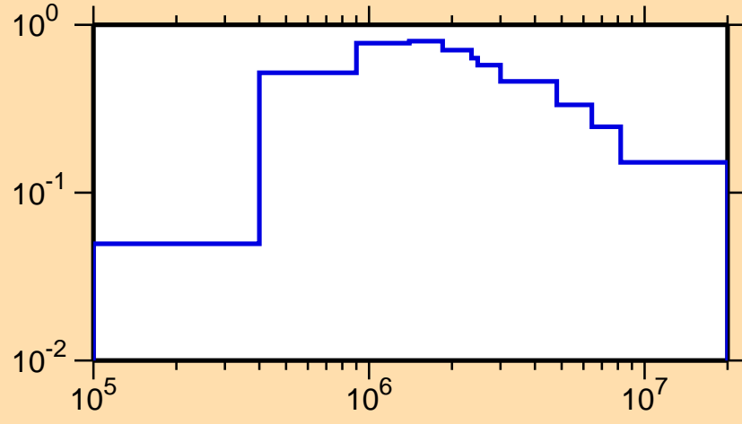
\sigma vs. E for ^{126}\text{Ba}(n,n_1)
