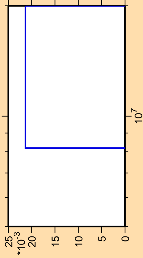
\Delta\sigma/\sigma vs. E for ^{126}\text{Ba}(\text{mt } 34)
