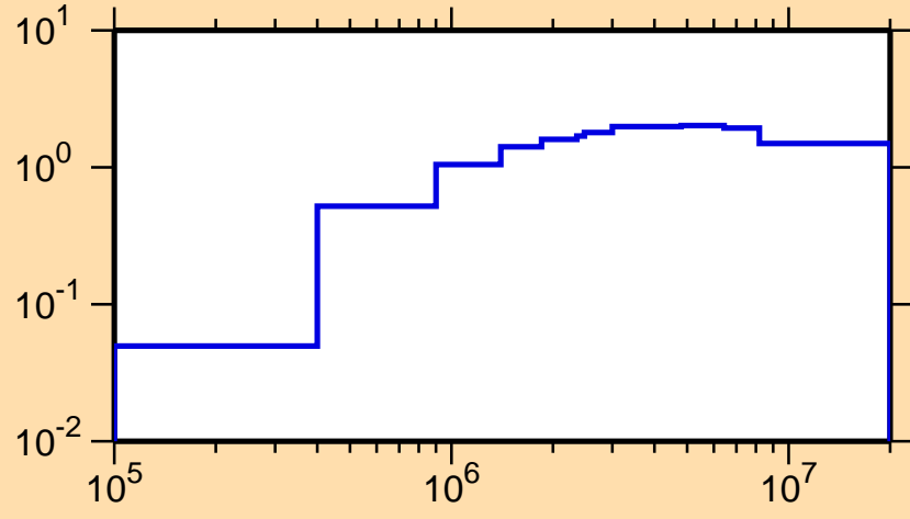
\sigma vs. E for ^{126}\text{Ba}(n,\text{inel.})
