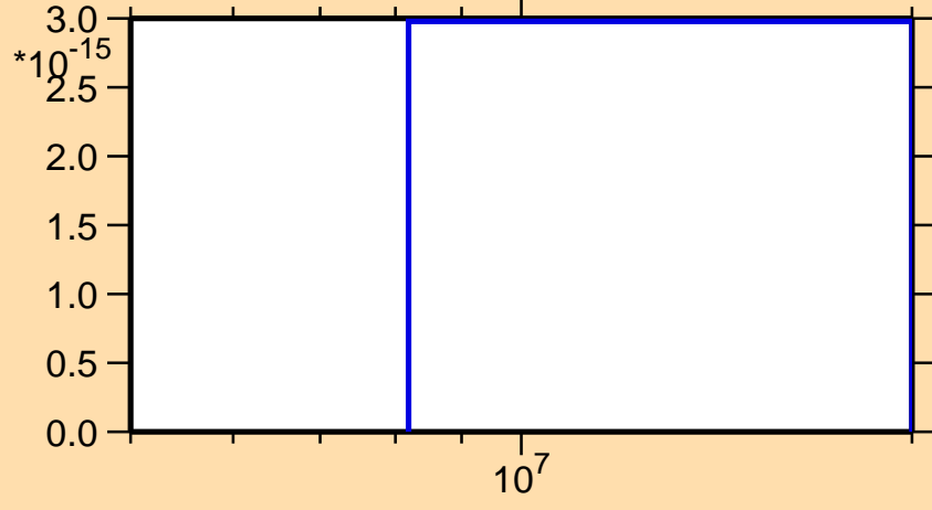
\sigma vs. E for ^{126}\text{Ba}(\text{mt } 34)
