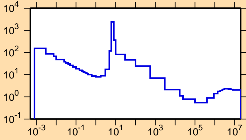
\sigma vs. E for ^{126}\text{Ba}(n,\text{nonel.})
