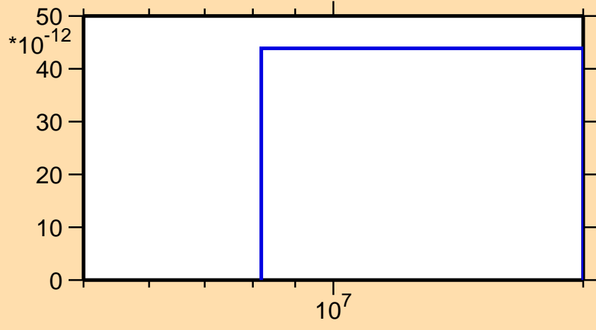
\sigma vs. E for ^{126}\text{Ba}(\text{mt } 45)
