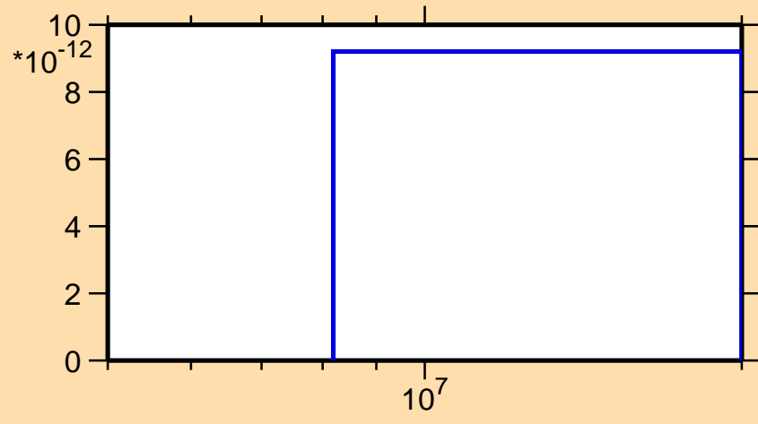
\sigma vs. E for ^{126}\text{Ba}(n,3n)
