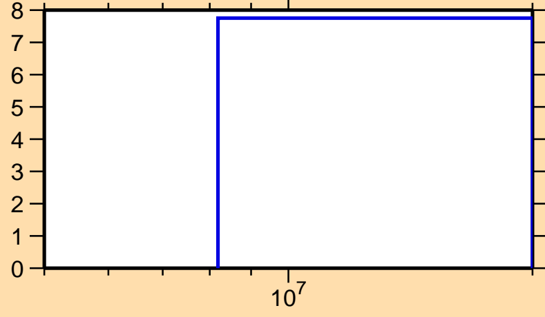
\Delta\sigma/\sigma vs. E for ^{126}\text{Ba}(n,\text{inel.})
