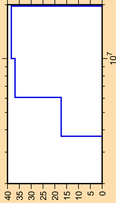
\Delta\sigma/\sigma vs. E for ^{127}\text{Ba}(n,n\alpha)
