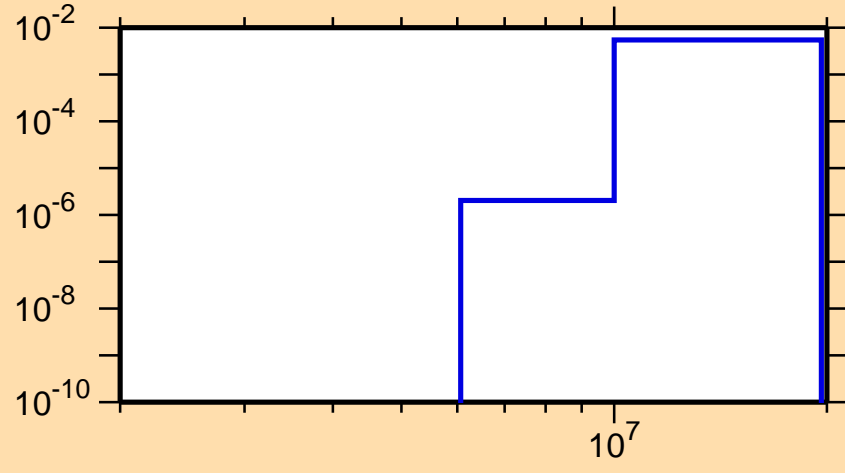
\sigma vs. E for ^{127}\text{Ba}(n,n\alpha)
