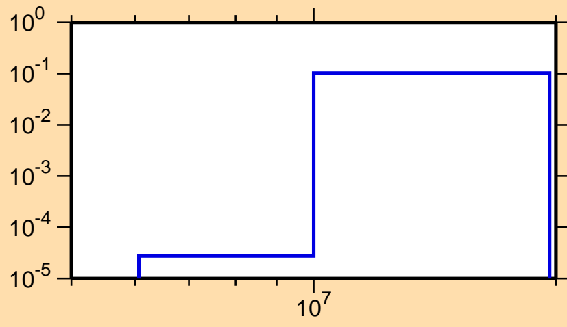
\sigma vs. E for ^{127}\text{Ba}(n,np)
