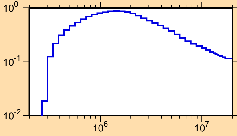
\sigma vs. E for ^{128}\text{Ba}(n,n_1)
