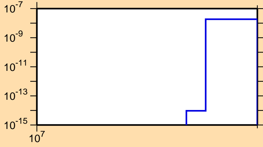
\sigma vs. E for ^{128}\text{Ba}(n,2np)
