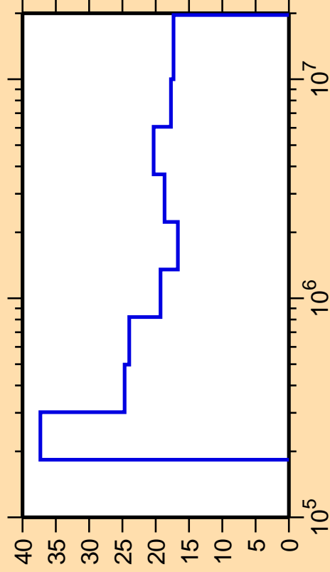
\Delta\sigma/\sigma vs. E for ^{128}\text{Ba}(n,n_1)
