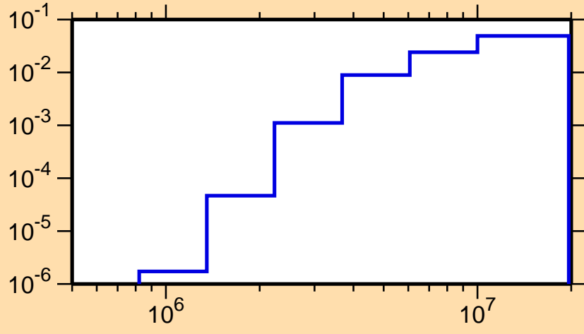
\sigma vs. E for ^{128}\text{Ba}(n,p)
