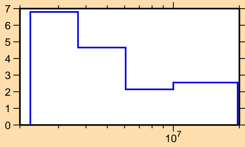
\Delta\sigma/\sigma vs. E for ^{128}\text{Ba}(n,\text{el.})
