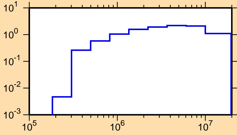
\sigma vs. E for ^{128}\text{Ba}(n,\text{inel.})
