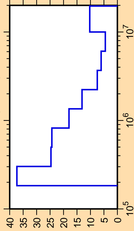
\Delta\sigma/\sigma vs. E for ^{128}\text{Ba}(n,\text{inel.})
