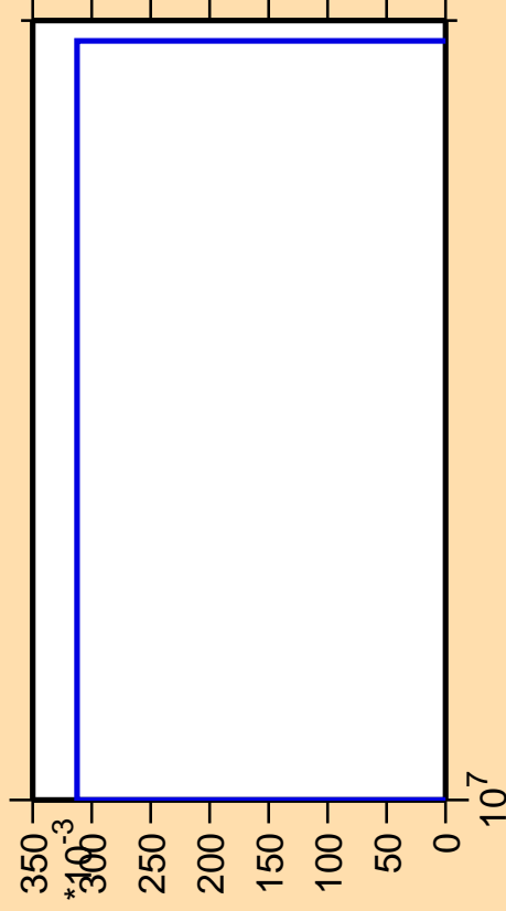
\Delta\sigma/\sigma vs. E for ^{128}\text{Ba} (mt 45)
