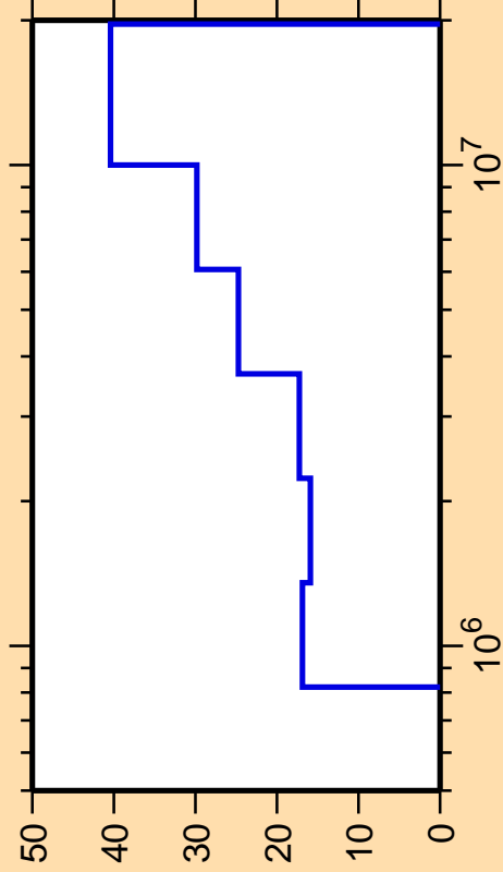
\Delta\sigma/\sigma vs. E for ^{128}\text{Ba}(n,n_4)
