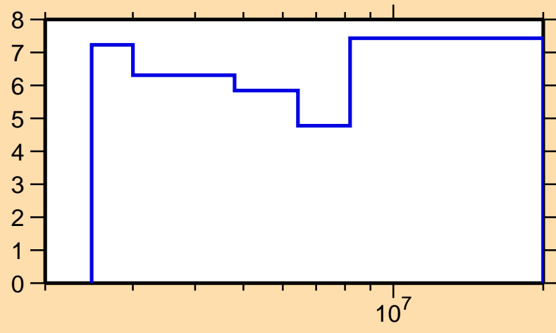
\Delta\sigma/\sigma vs. E for ^{128}\text{Ba}(n,\text{inel.})
