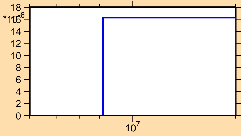
\sigma vs. E for ^{128}\text{Ba}(n,t)
