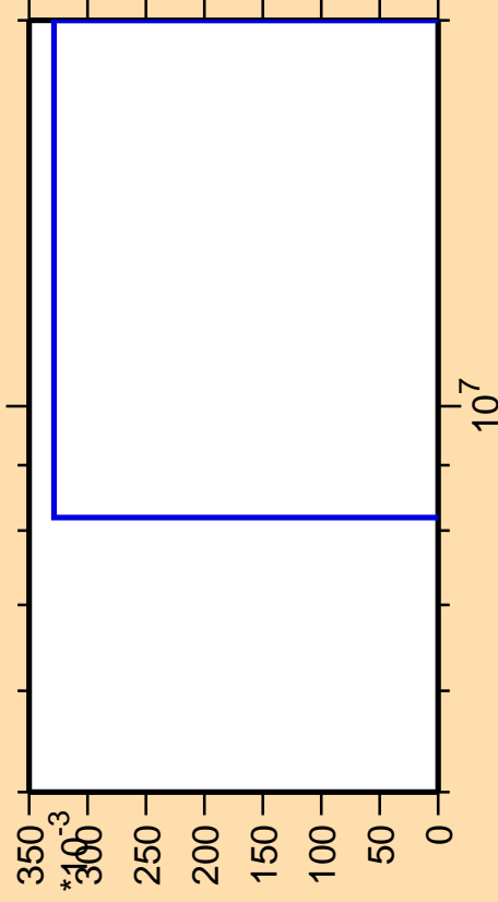
\Delta\sigma/\sigma vs. E for ^{128}\text{Ba}(\text{mt } 45)
