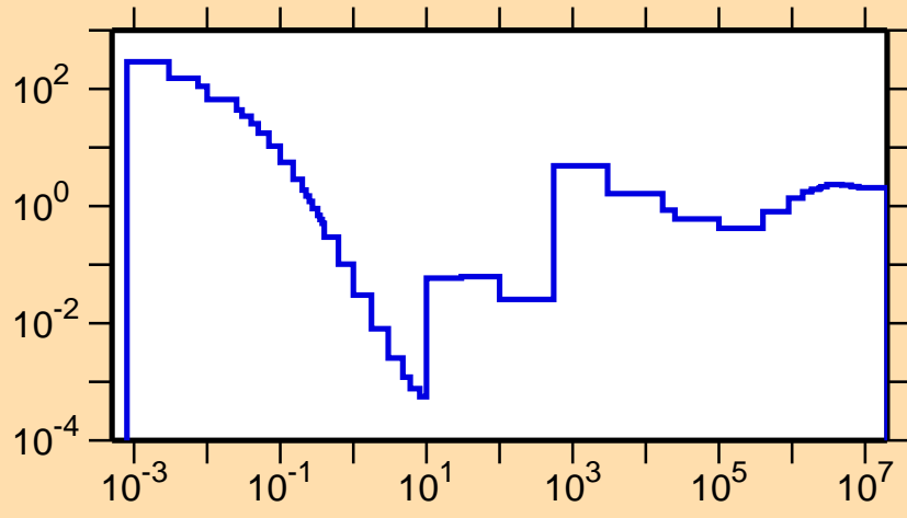
\sigma vs. E for ^{128}\text{Ba}(n,\text{nonel.})
