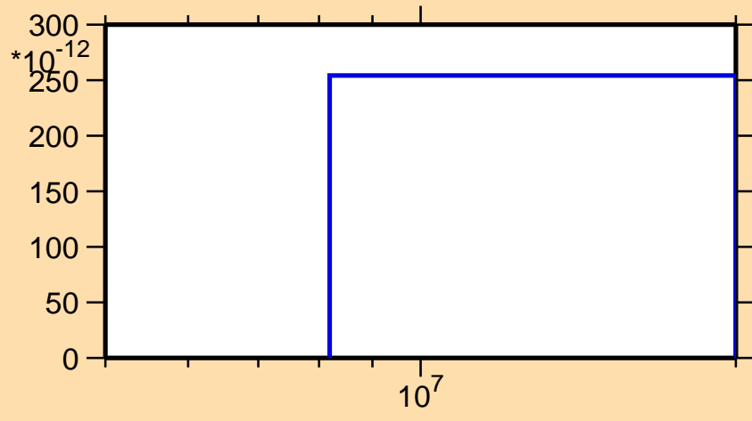
\sigma vs. E for ^{128}\text{Ba}(n,\text{nd})
