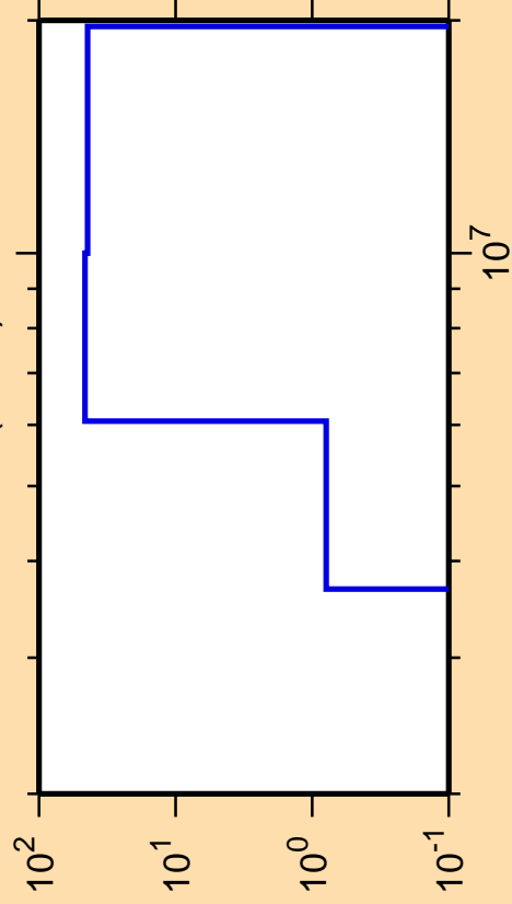
\Delta\sigma/\sigma vs. E for ^{129}\text{Ba}(n,n\alpha)
