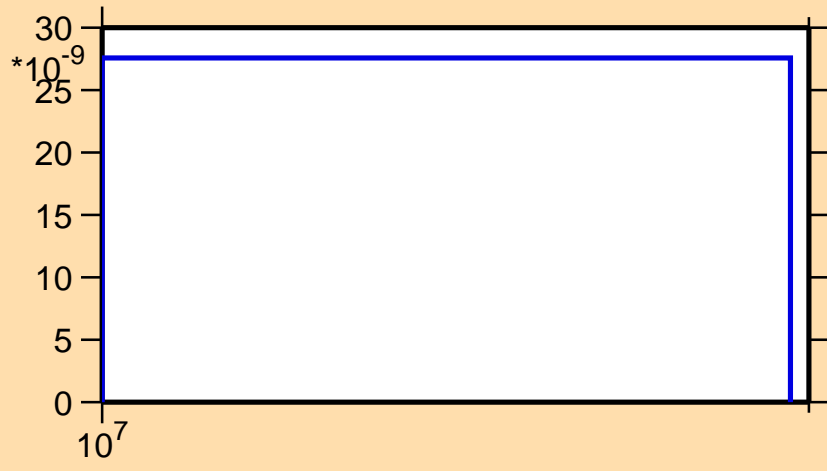
\sigma vs. E for ^{129}\text{Ba}(n,2n\alpha)
