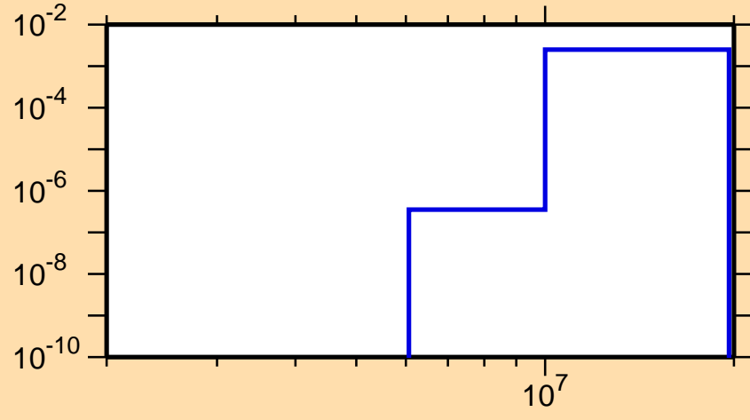
\sigma vs. E for ^{129}\text{Ba}(n,n\alpha)
