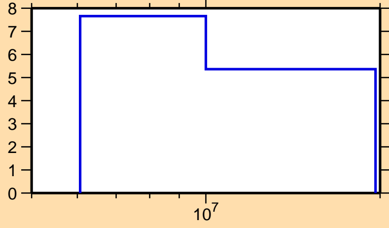
\Delta\sigma/\sigma vs. E for ^{129}\text{Ba}(n,2n)
