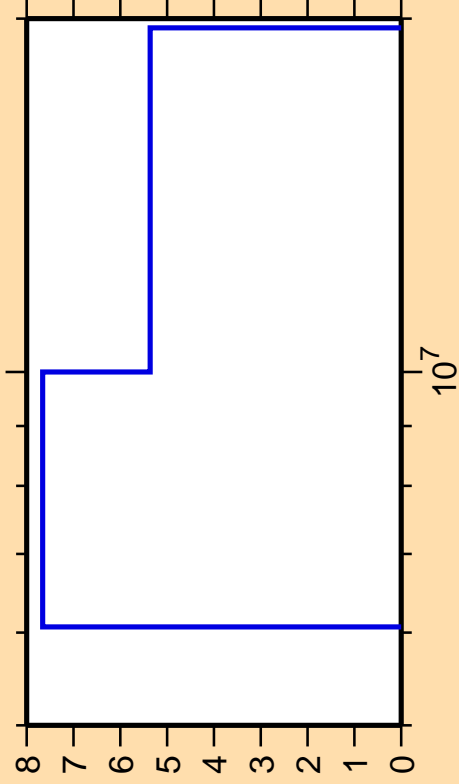
\Delta\sigma/\sigma vs. E for ^{129}\text{Ba}(n,2n)
