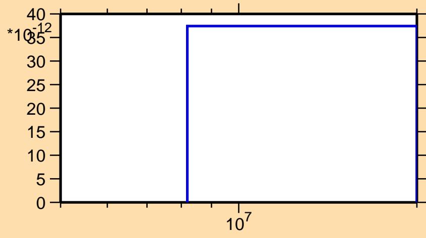
\sigma vs. E for ^{129}\text{Ba}(n,pd)
