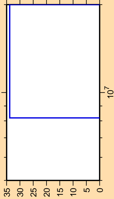
\Delta\sigma/\sigma vs. E for ^{129}\text{Ba}(n,pd)
