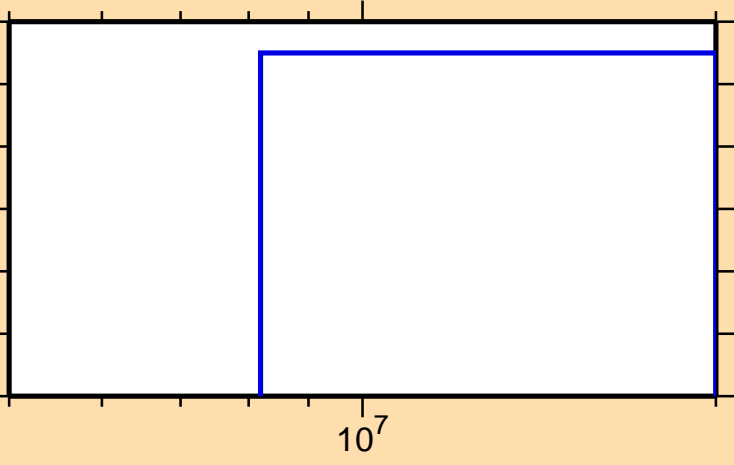
\sigma vs. E for ^{129}\text{Ba}(n,\text{pt})
