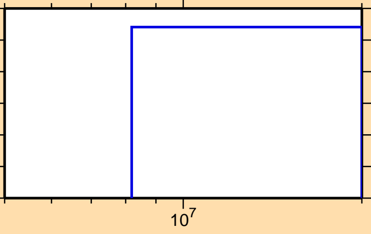
\sigma vs. E for ^{129}\text{Ba}(\text{mt117})
