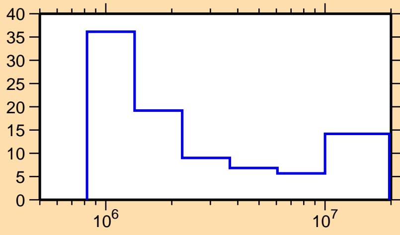
\Delta\sigma/\sigma vs. E for ^{131}\text{Ba}(n,n\text{cont.})
