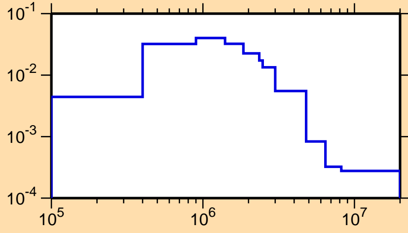
\sigma vs. E for ^{131}\text{Ba}(n,n_2)
