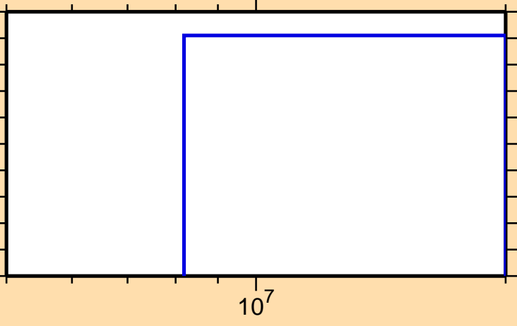
\sigma vs. E for ^{131}\text{Ba}(n,p\alpha)
