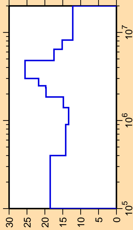
\Delta\sigma/\sigma vs. E for ^{131}\text{Ba}(n,n_2)
