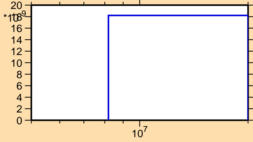
\sigma vs. E for ^{131}\text{Ba}(n,p\alpha)
